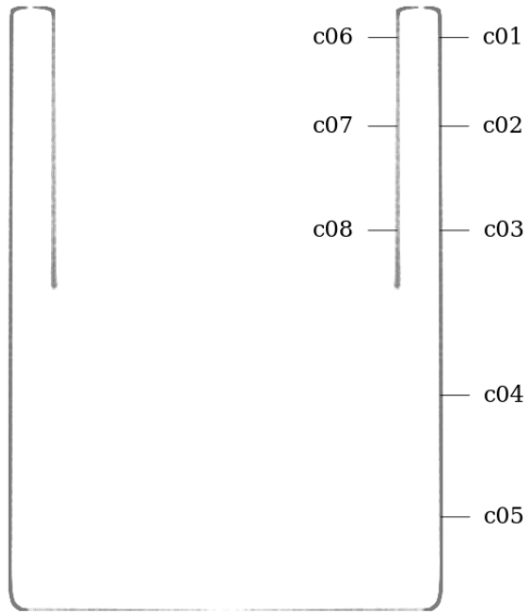
Figure 66: Circularicity measurement sample locations, full mesh aligned to exterior surface
