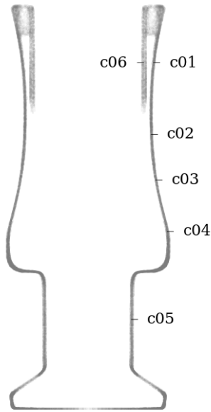
Figure 74: Circularity measurement sample locations, full mesh aligned to exterior surface
