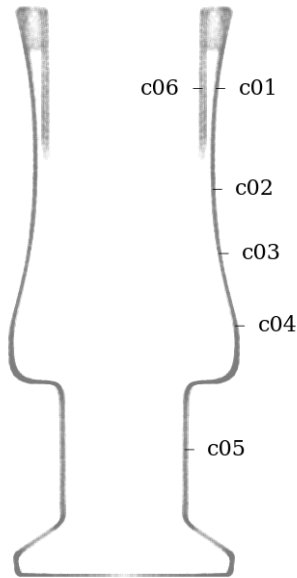
Figure 72: Circularity measurement sample locations, full mesh aligned to exterior surface
