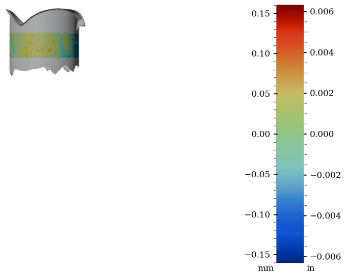
Figure 52: Surface variability heatmap of IV016, rotated 270°
