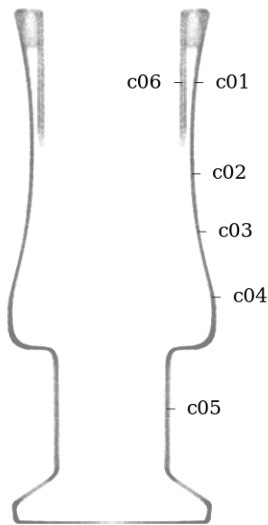
Figure 29: Circularity measurement sample locations, full mesh aligned to exterior surface
