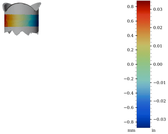
Figure 47: Surface variability heatmap of IV016, rotated 180°
