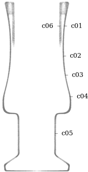
Figure 56: Circularity measurement sample locations, full mesh aligned to exterior surface
