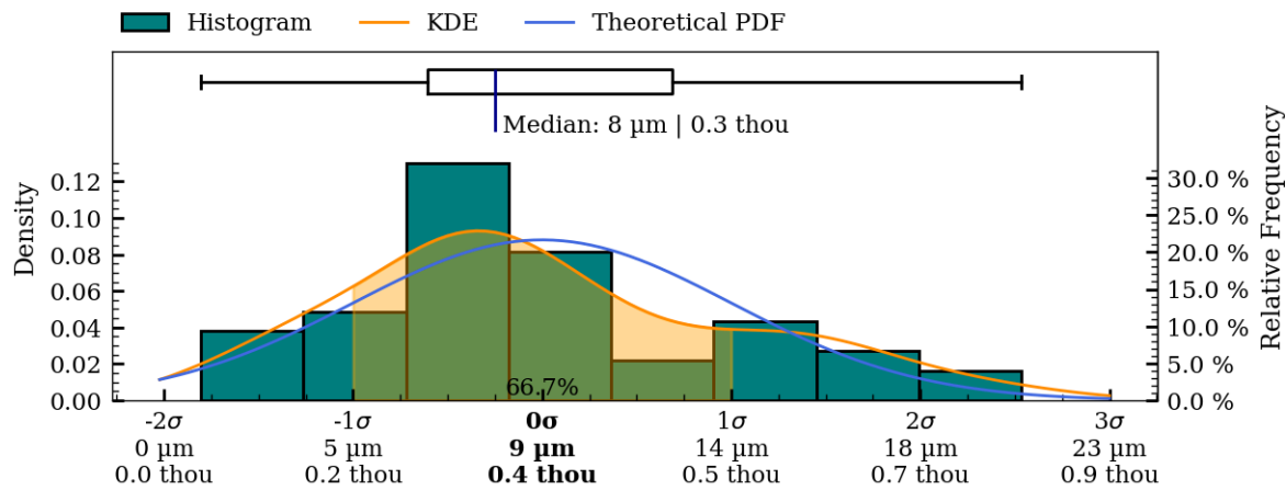
Figure 40: Coaxiality residual plots of interior_separate surface, IV016.
