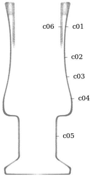
Figure 58: Circularity measurement sample locations, full mesh aligned to exterior surface
