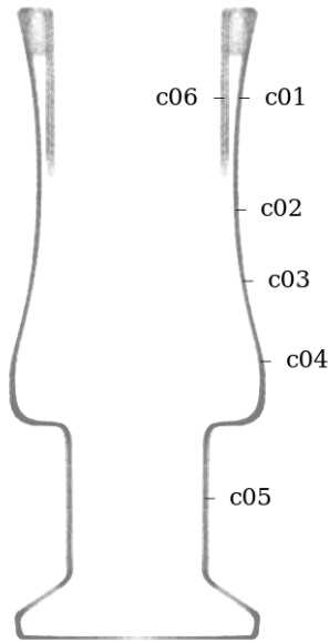
Figure 4: Circularity measurement sample locations, full mesh aligned with exterior surface
