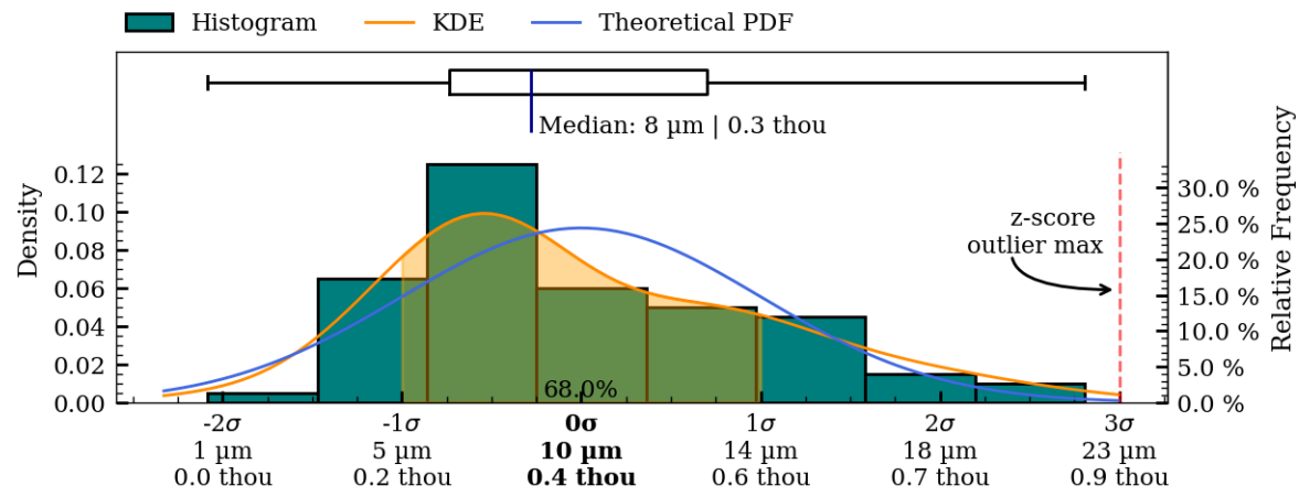
Figure 39: Coaxiality residual plots of interior surface, IV016.
