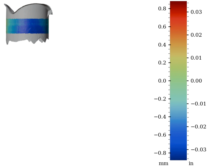
Figure 48: Surface variability heatmap of IV016, rotated 270°
