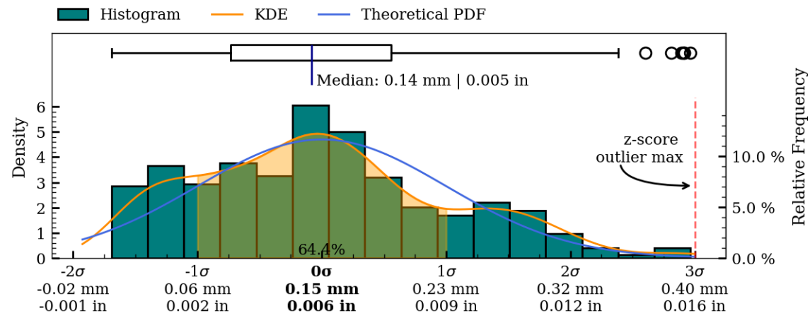
Figure 38: Coaxiality residual plots of exterior surface, IV016.
