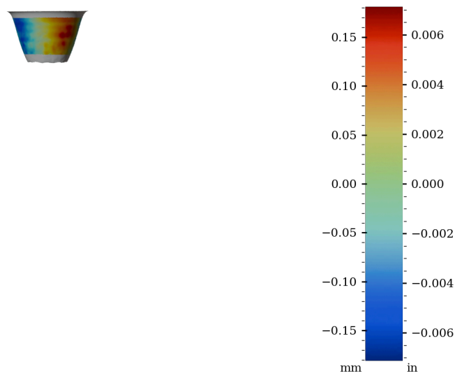
Figure 51: Surface variability heatmap of IV015, rotated 180°
