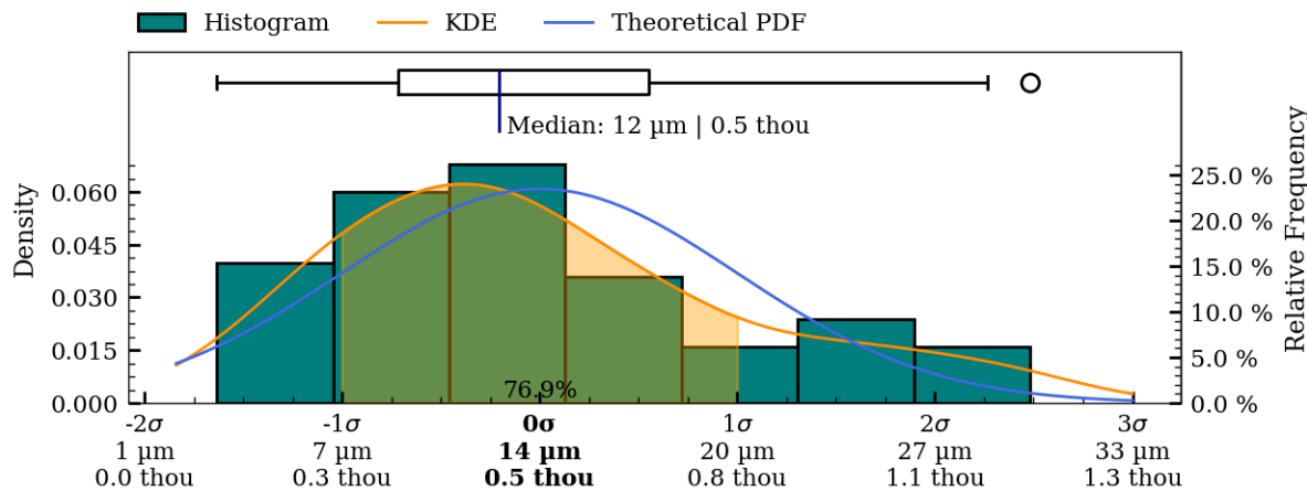
Figure 39: Coaxiality residual plots of interior surface, IV015.
