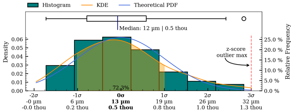
Figure 40: Coaxiality residual plots of interior_separate surface, IV015.
