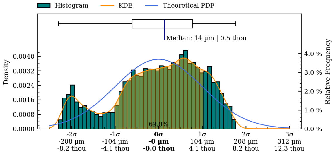
Figure 54: Interior surface variability boxplot, kds and histogram.
