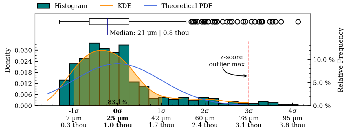
Figure 38: Coaxiality residual plots of exterior surface, IV015.
