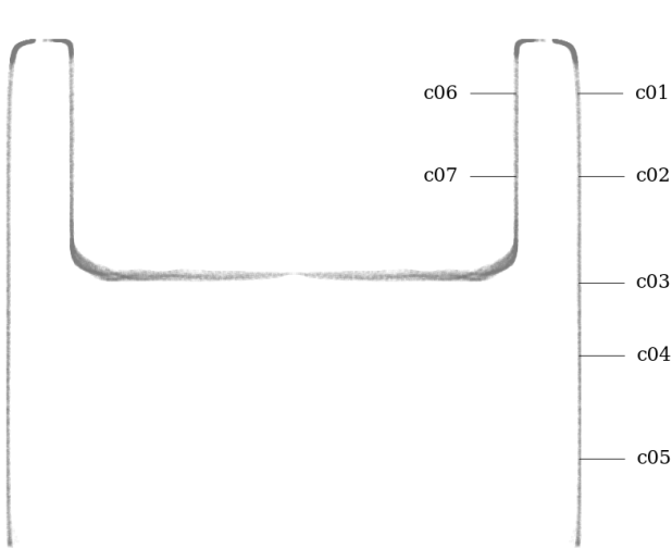
Figure 60: Circularity measurement sample locations, full mesh aligned to exterior surface
