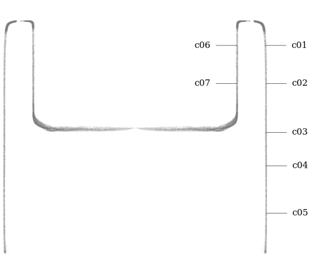
Figure 62: Circularity measurement sample locations, full mesh aligned to exterior surface
