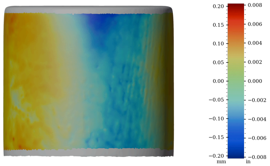
Figure 47: Surface variability heatmap of IV011, rotated 180°
