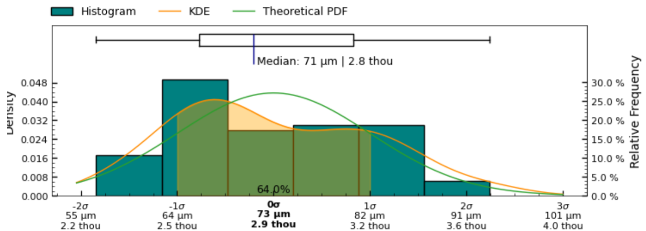
Figure 24: Root Mean Squared Deviation measurement distribution across measured slices of interior surface
