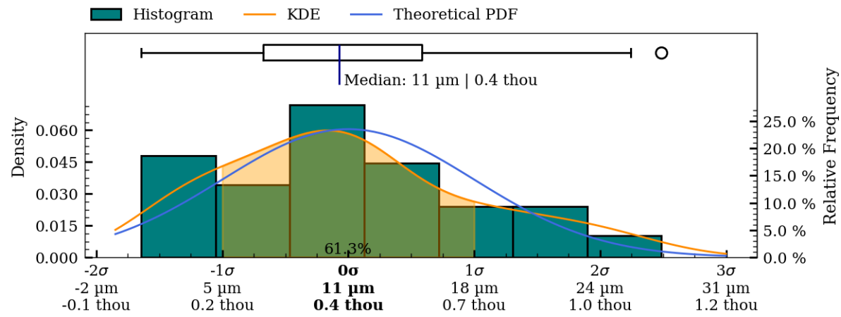
Figure 43: Coaxiality residual plots of interior surface, IV011.
