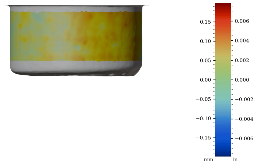
Figure 51: Surface variability heatmap of IV011, rotated 180°
