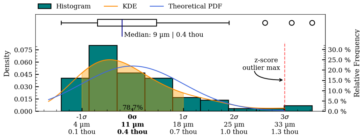
Figure 44: Coaxiality residual plots of interior_separate surface, IV011.
