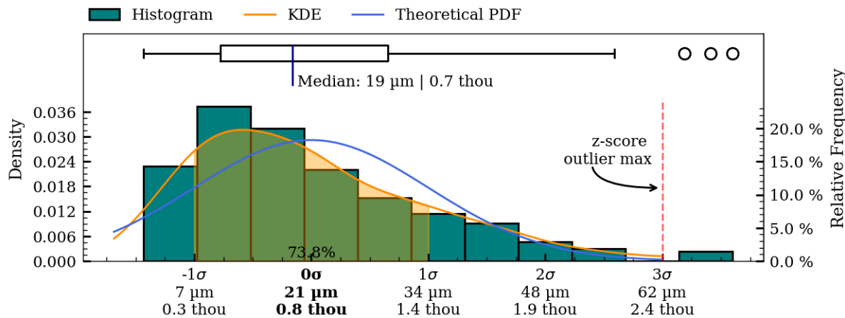
Figure 42: Coaxiality residual plots of exterior surface, IV011.
