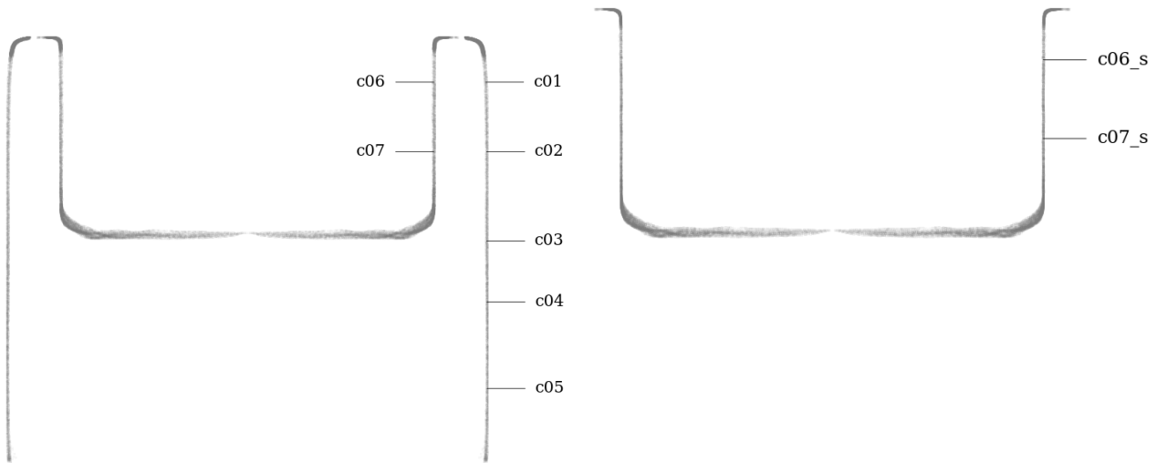
Figure 78: Circularity measurement sample locations, full mesh aligned to exterior surface
