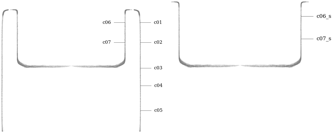
Figure 31: Circularity measurement sample locations, full mesh aligned to exterior surface
