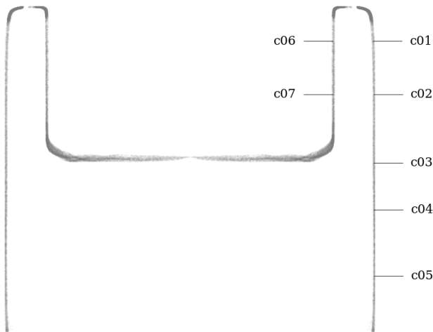
Figure 76: Circularity measurement sample locations, full mesh aligned to exterior surface
