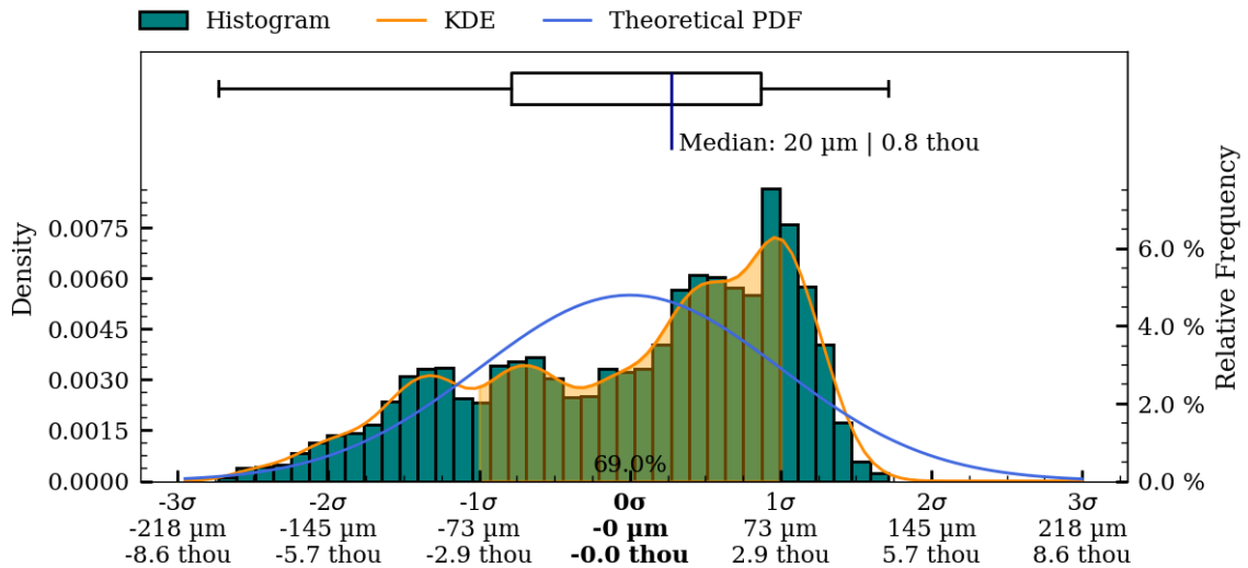
Figure 58: Interior surface variability boxplot, kds and histogram.
