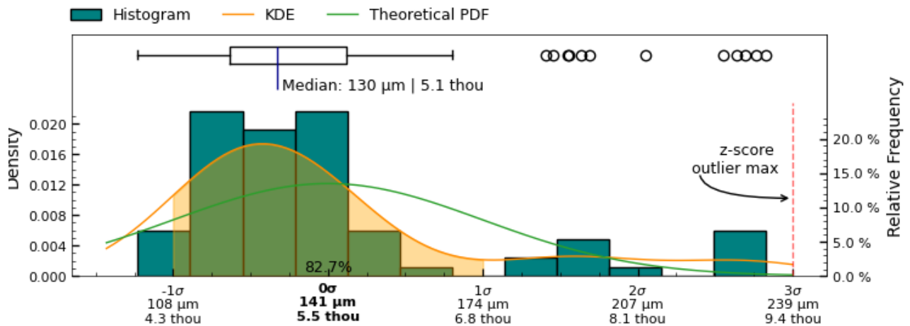
Figure 27: Range measurement distribution across measured slices of interior_separate surface
