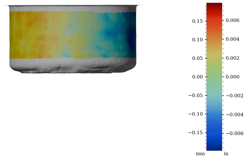
Figure 52: Surface variability heatmap of IV011, rotated 270°
