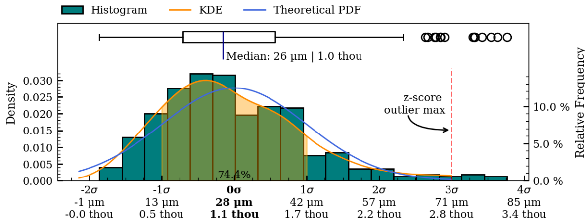
Figure 42: Coaxiality residual plots of exterior surface, IV010.
