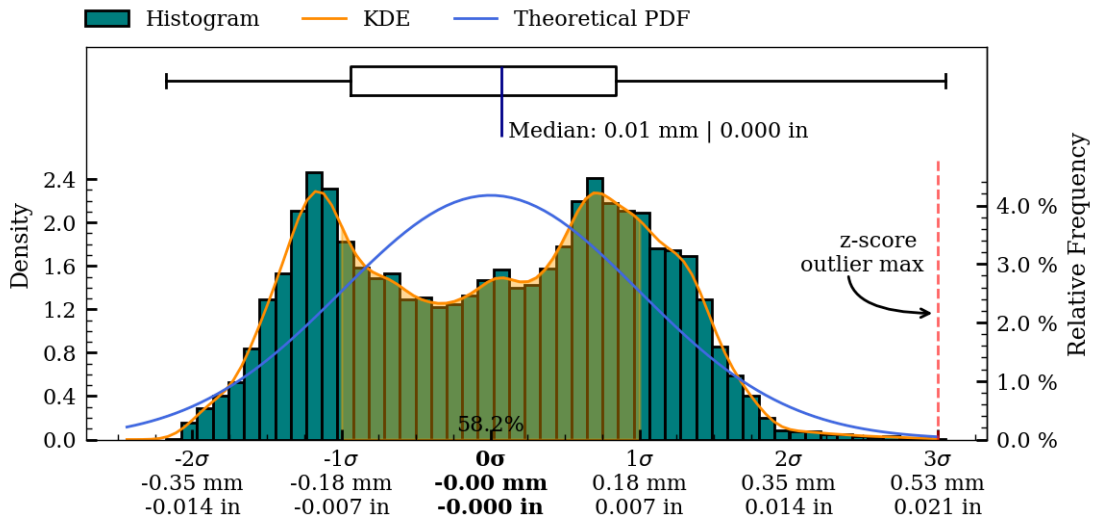
Figure 58: Interior surface variability boxplot, kds and histogram.
