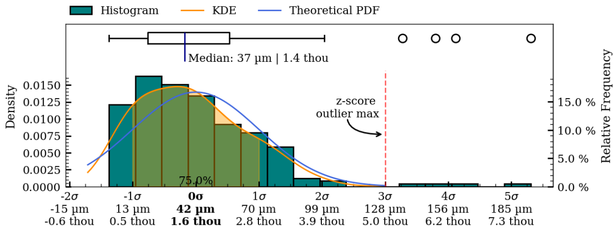
Figure 43: Coaxiality residual plots of interior surface, IV010.
