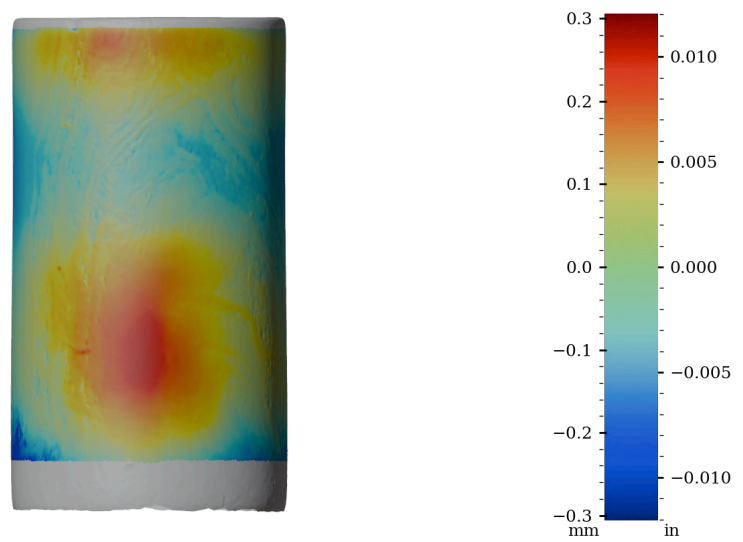
Figure 48: Surface variability heatmap of IV010, rotated 270°
