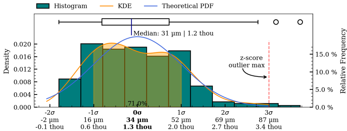
Figure 44: Coaxiality residual plots of interior_separate surface, IV010.
