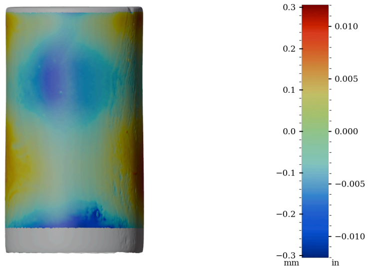
Figure 47: Surface variability heatmap of IV010, rotated 180°
