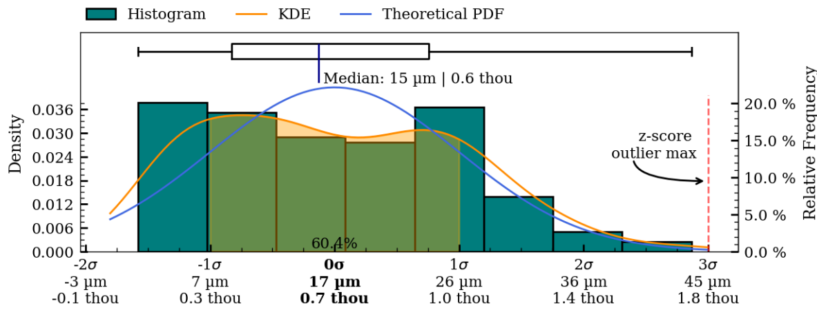
Figure 44: Coaxiality residual plots of interior_separate surface, IV008.
