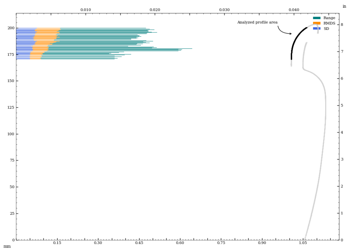
Figure 68: Circularity of interior surface - perpendicular to surface curvature.
