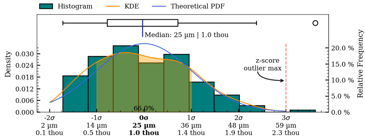
Figure 43: Coaxiality residual plots of interior surface, IV008.
