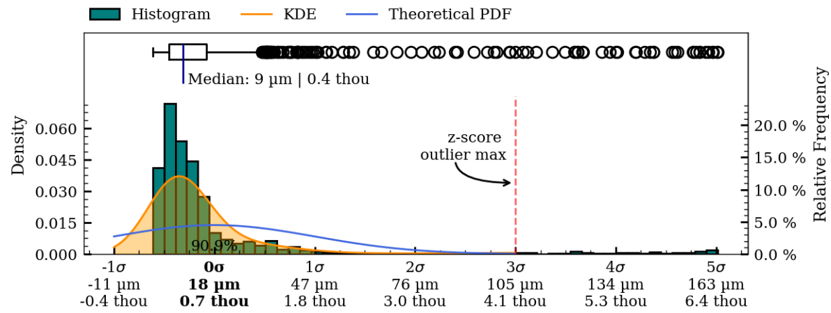
Figure 42: Coaxiality residual plots of exterior surface, IV008.
