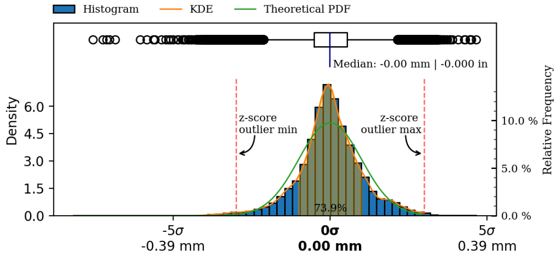
Figure 57: Exterior surface variability boxplot, kds and histogram.
