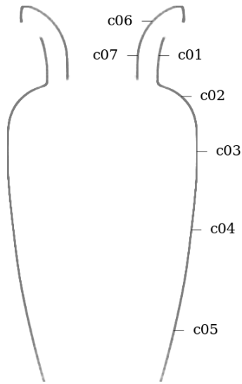
Figure 76: Circularity measurement sample locations, full mesh aligned to exterior surface
