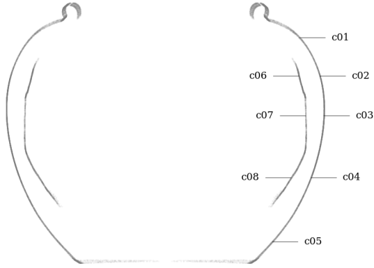
Figure 4: Circularity measurement sample locations, full mesh aligned with exterior surface
