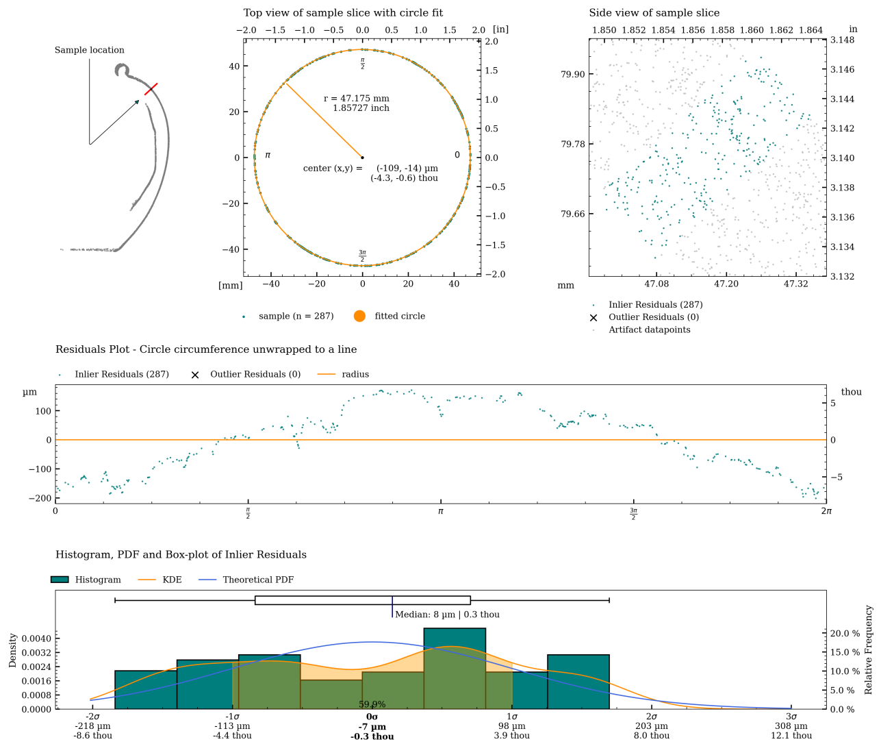
Figure 35: Detailed plot of concentricity measurement for c01.
