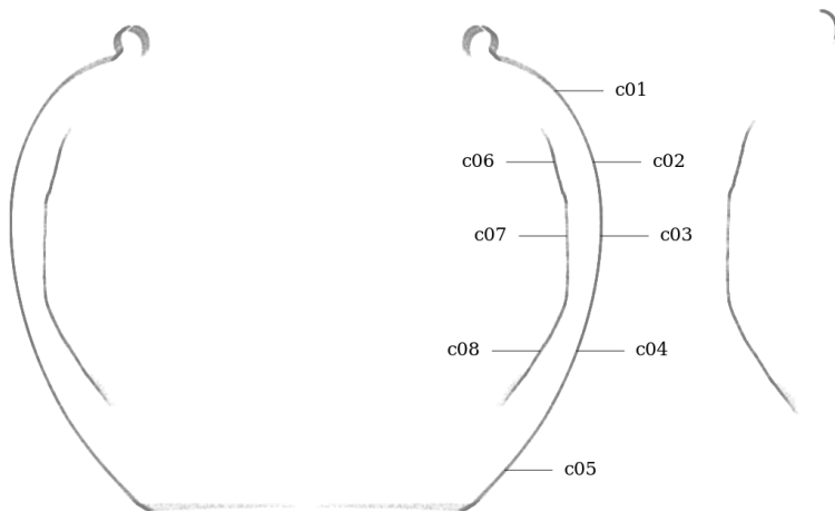
Figure 66: Circularity measurement sample locations, full mesh aligned to exterior surface
