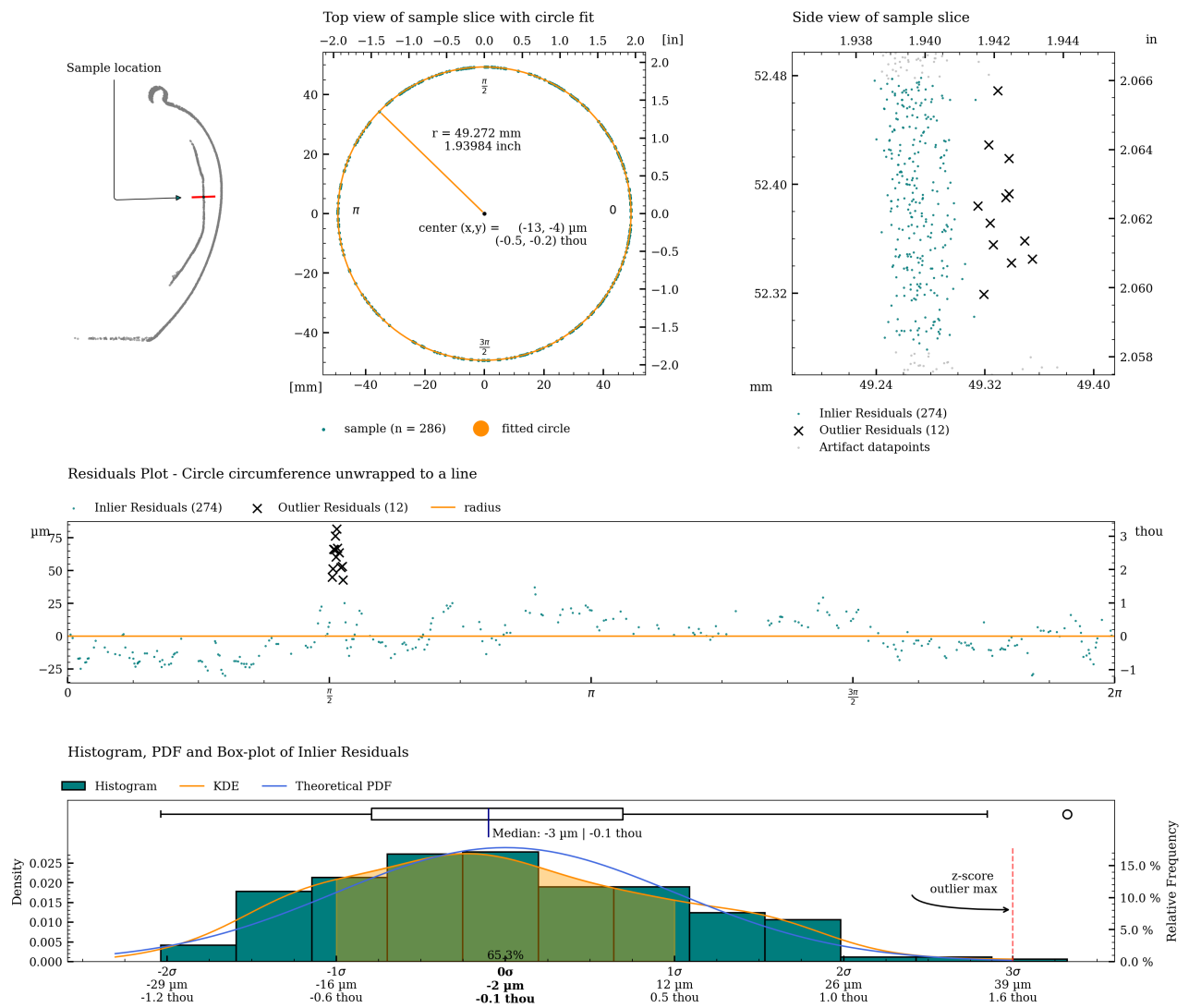
Figure 43: Detailed plot of concentricity measurement for c07_s.
