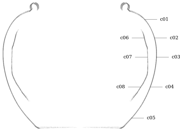
Figure 33: Circularity measurement sample locations, full mesh aligned to exterior surface
