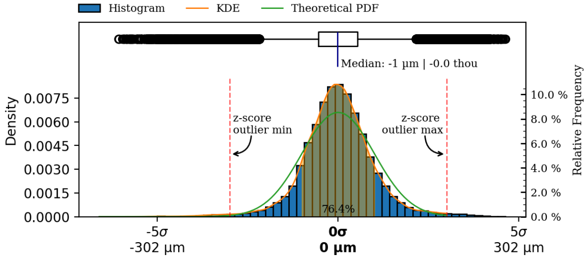
Figure 61: Exterior surface variability boxplot, kds and histogram.
