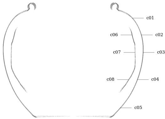
Figure 82: Circularity measurement sample locations, full mesh aligned to exterior surface
