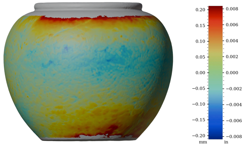
Figure 52: Surface variability heatmap of IV007, rotated 270°
