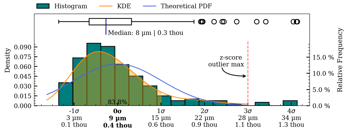
Figure 48: Coaxiality residual plots of interior_separate surface, IV007.
