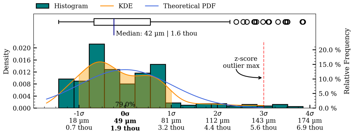
Figure 46: Coaxiality residual plots of exterior surface, IV007.
