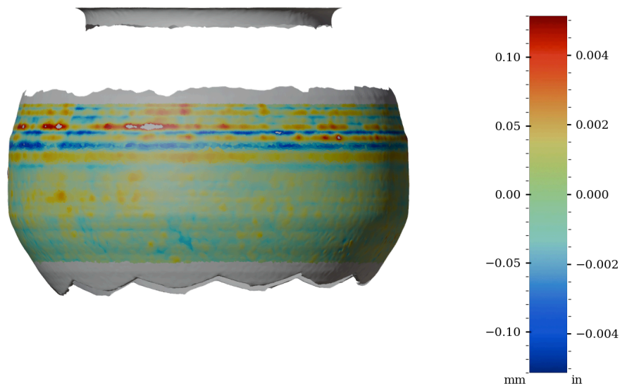
Figure 60: Surface variability heatmap of IV007, rotated 270°
