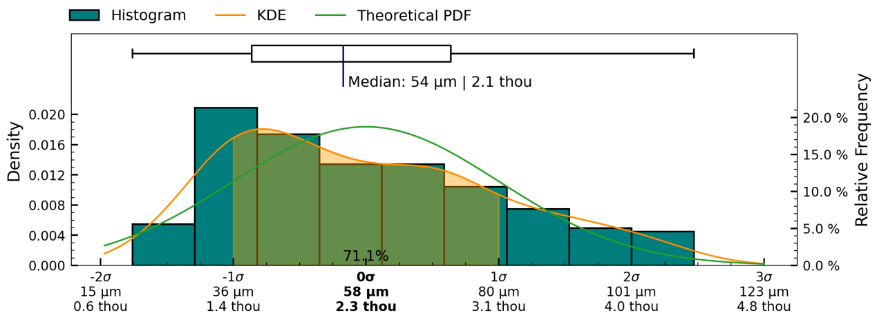
Figure 26: Root Mean Squared Deviation measurement distribution across measured slices of interior surface
