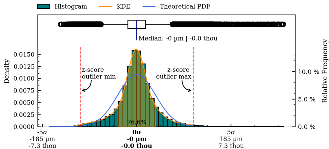
Figure 63: Interior separately aligned surface variability boxplot, kds and histogram.
