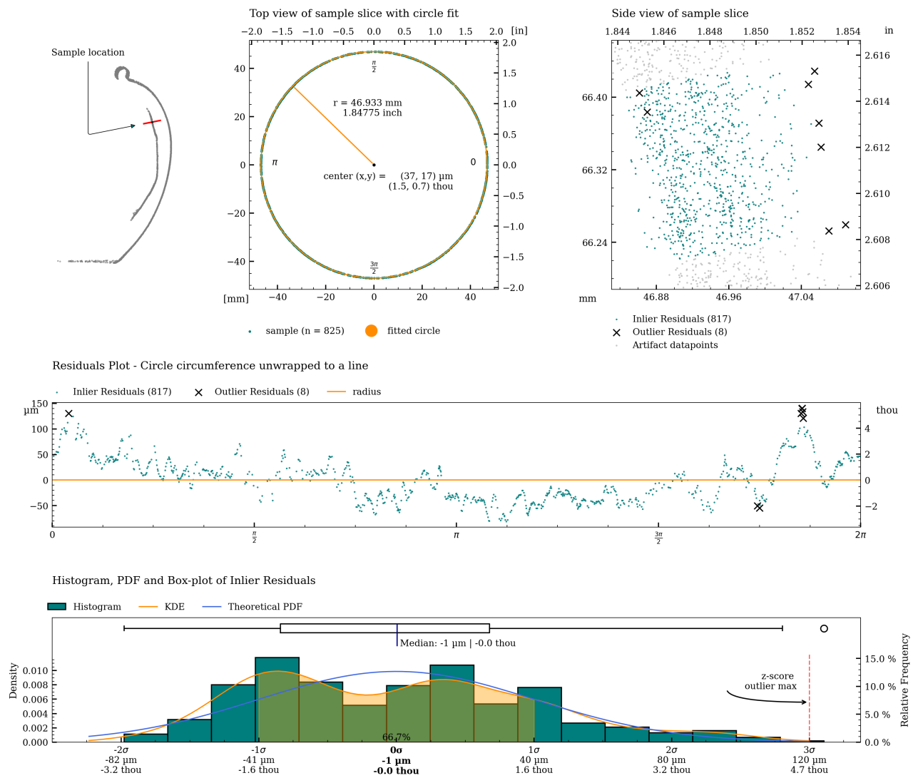
Figure 40: Detailed plot of concentricity measurement for c06.
