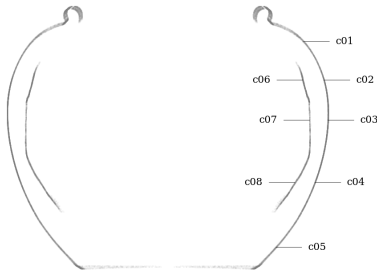
Figure 80: Circularity measurement sample locations, full mesh aligned to exterior surface
