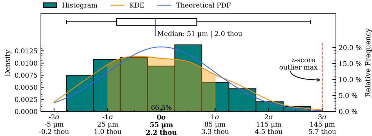
Figure 47: Coaxiality residual plots of interior surface, IV007.
