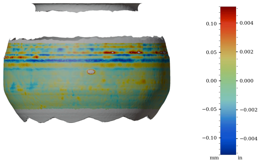
Figure 59: Surface variability heatmap of IV007, rotated 180°
