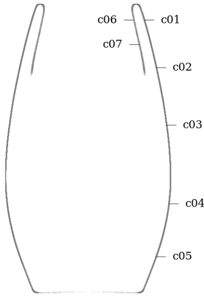
Figure 60: Circularity measurement sample locations, full mesh aligned to exterior surface
