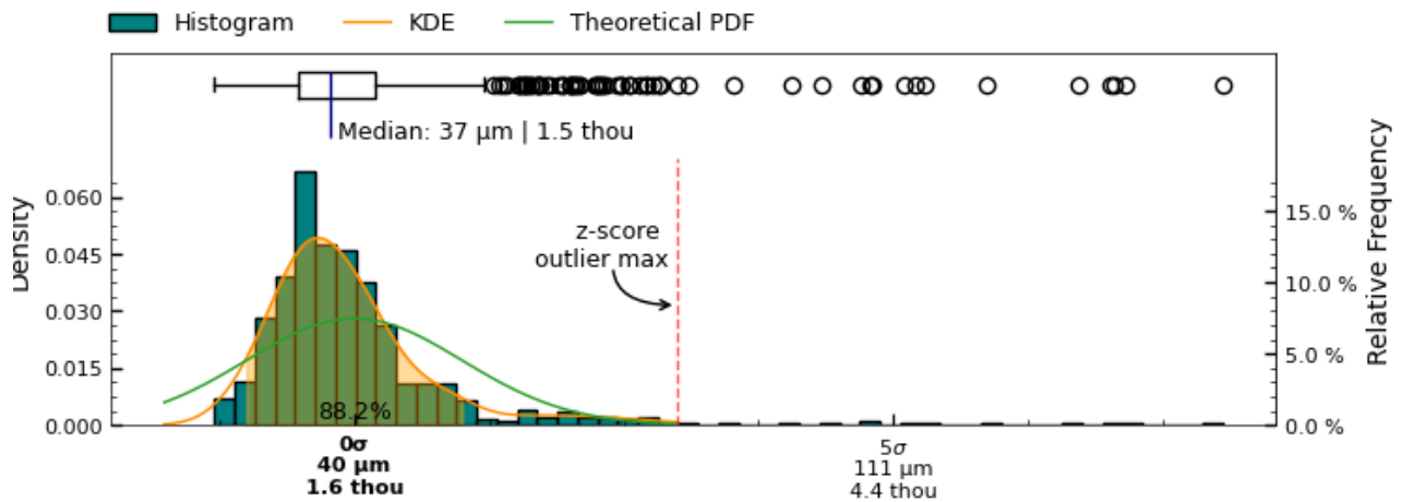
Figure 19: Root Mean Squared Deviation measurement distribution across measured slices of exterior surface
