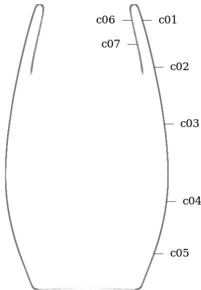
Figure 31: Circularity measurement sample locations, full mesh aligned to exterior surface
