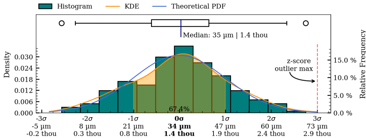
Figure 44: Coaxiality residual plots of interior_separate surface, IV004.
