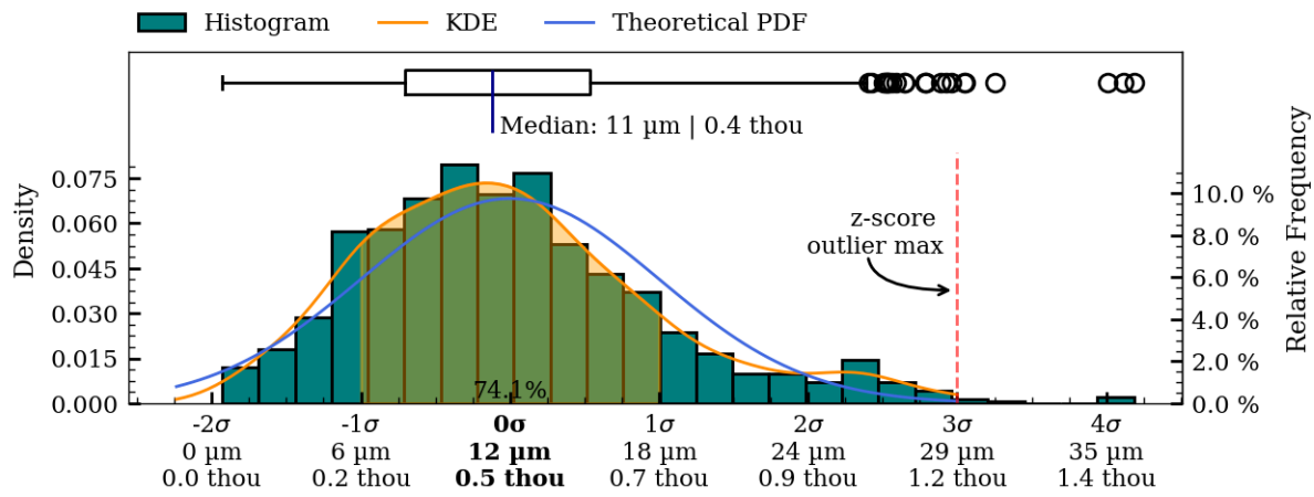
Figure 42: Coaxiality residual plots of exterior surface, IV004.
