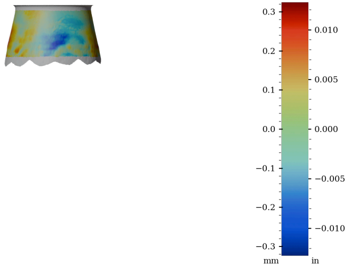
Figure 55: Surface variability heatmap of IV004, rotated 180°
