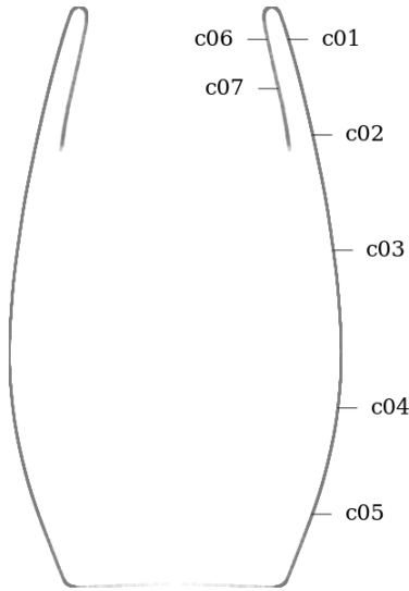
Figure 76: Circularity measurement sample locations, full mesh aligned to exterior surface
