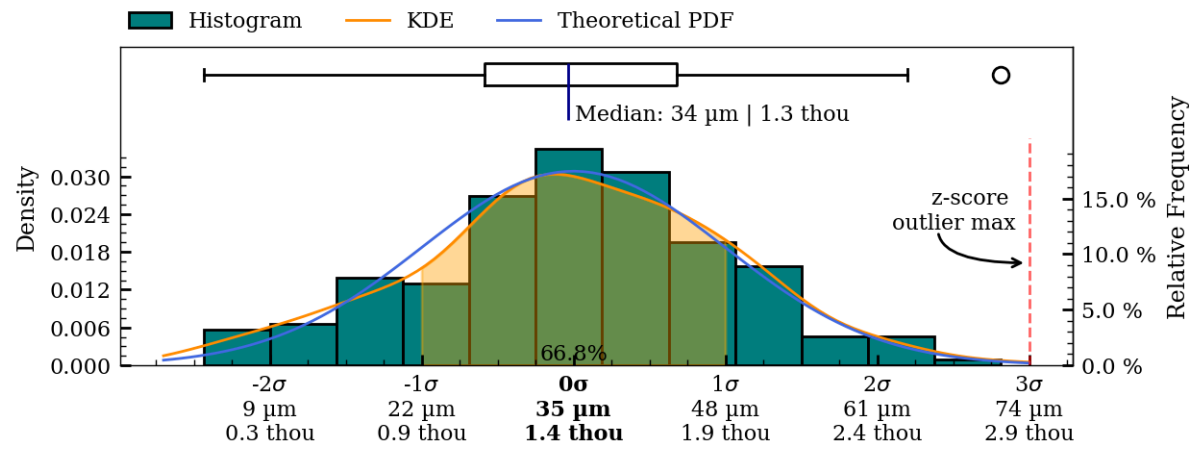
Figure 43: Coaxiality residual plots of interior surface, IV004.
