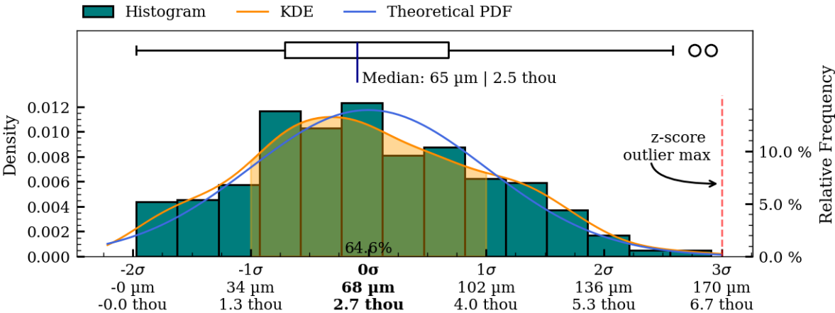
Figure 55: Coaxiality residual plots of interior surface, IV002.
