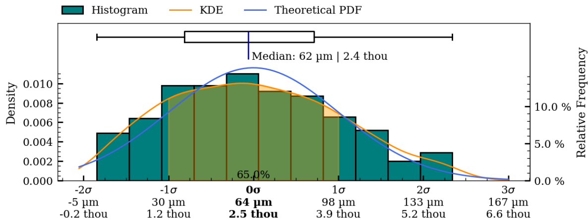
Figure 56: Coaxiality residual plots of interior_separate surface, IV002.
