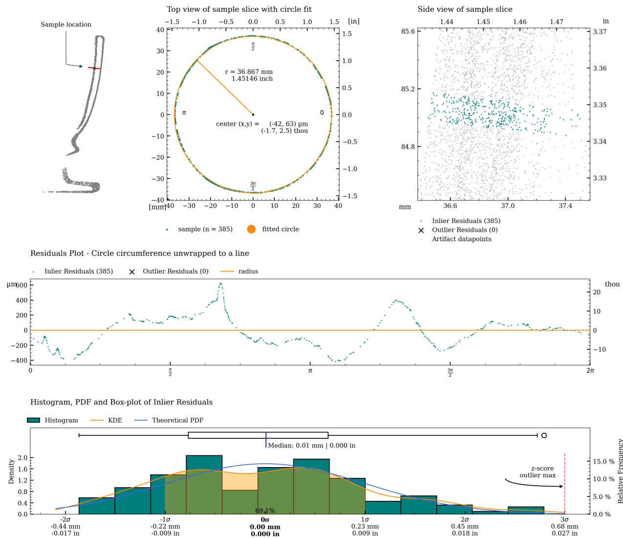
Figure 43: Detailed plot of concentricity measurement for c07_s.
