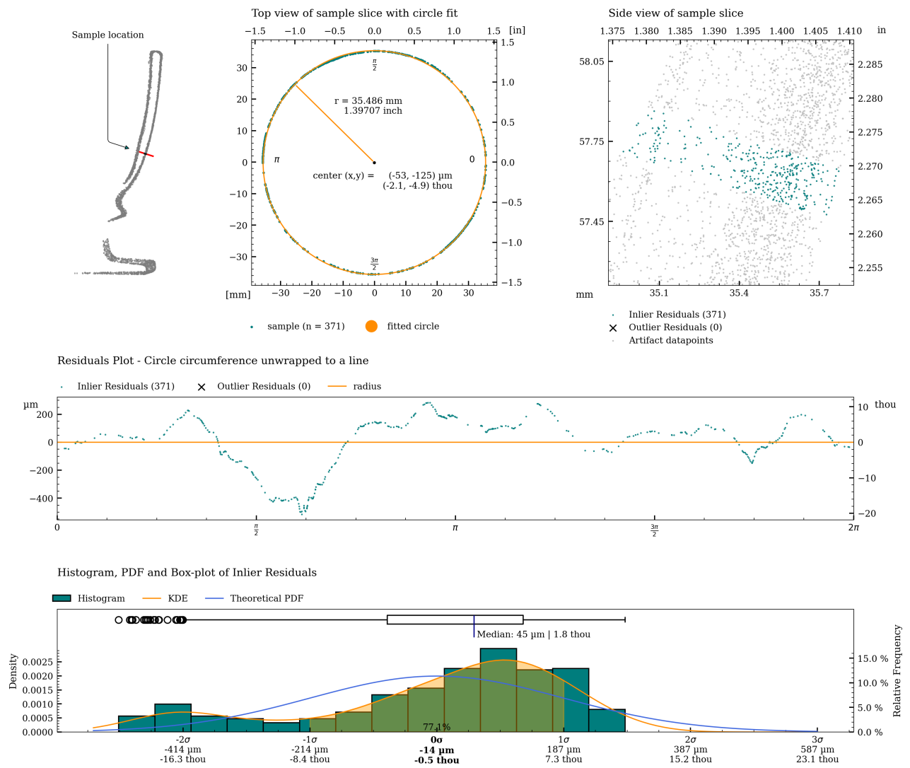
Figure 38: Detailed plot of concentricity measurement for c04.
