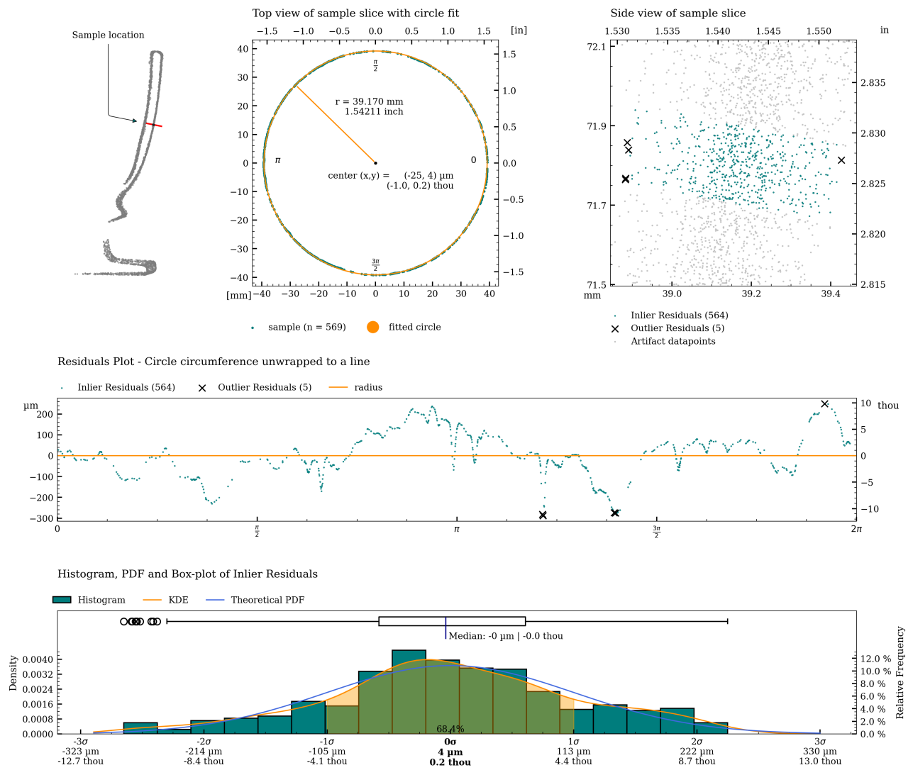
Figure 37: Detailed plot of concentricity measurement for c03.
