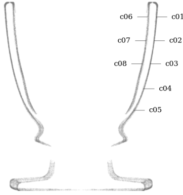
Figure 4: Circularity measurement sample locations, full mesh aligned with exterior surface
