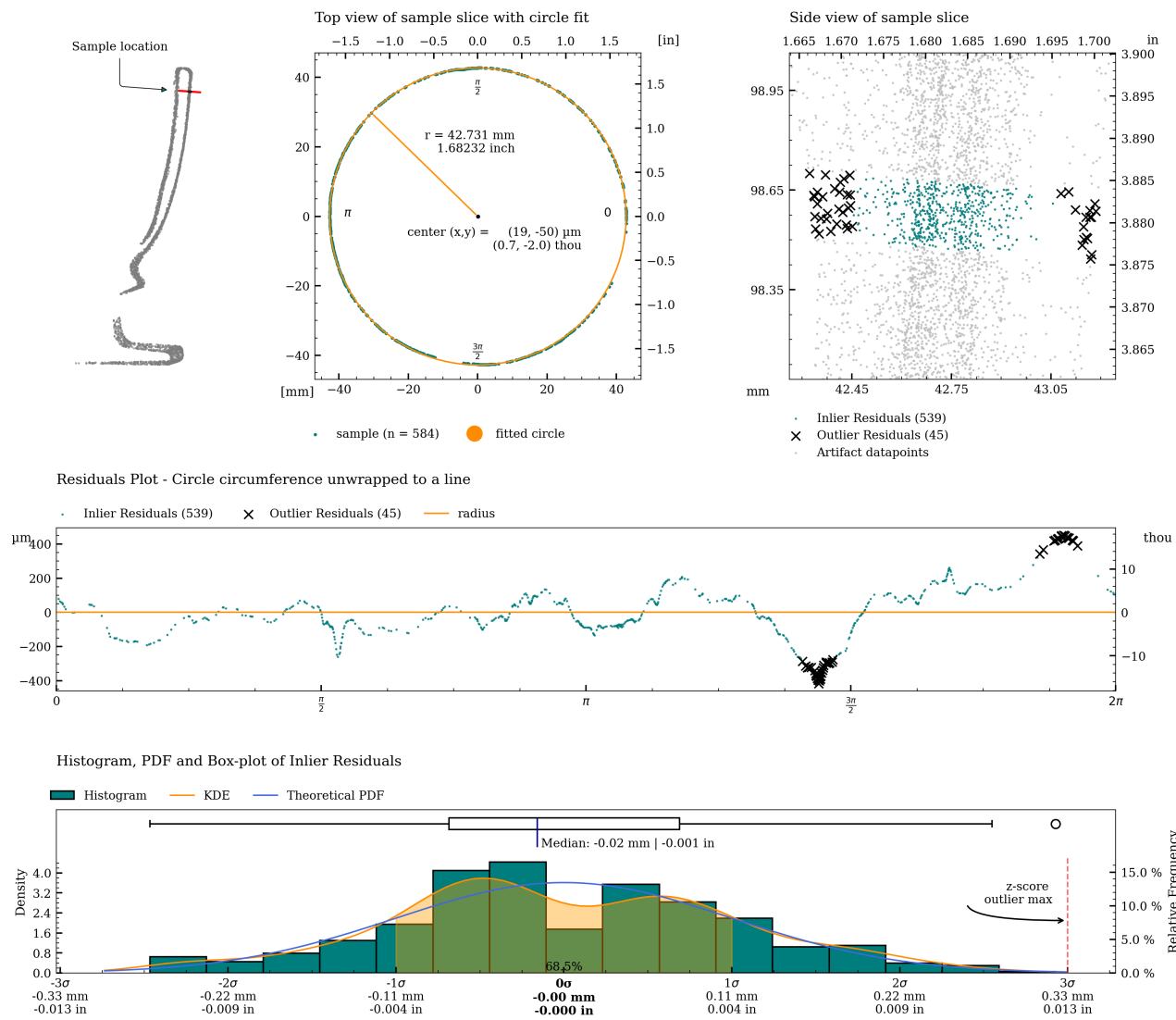
Figure 35: Detailed plot of concentricity measurement for c01.
