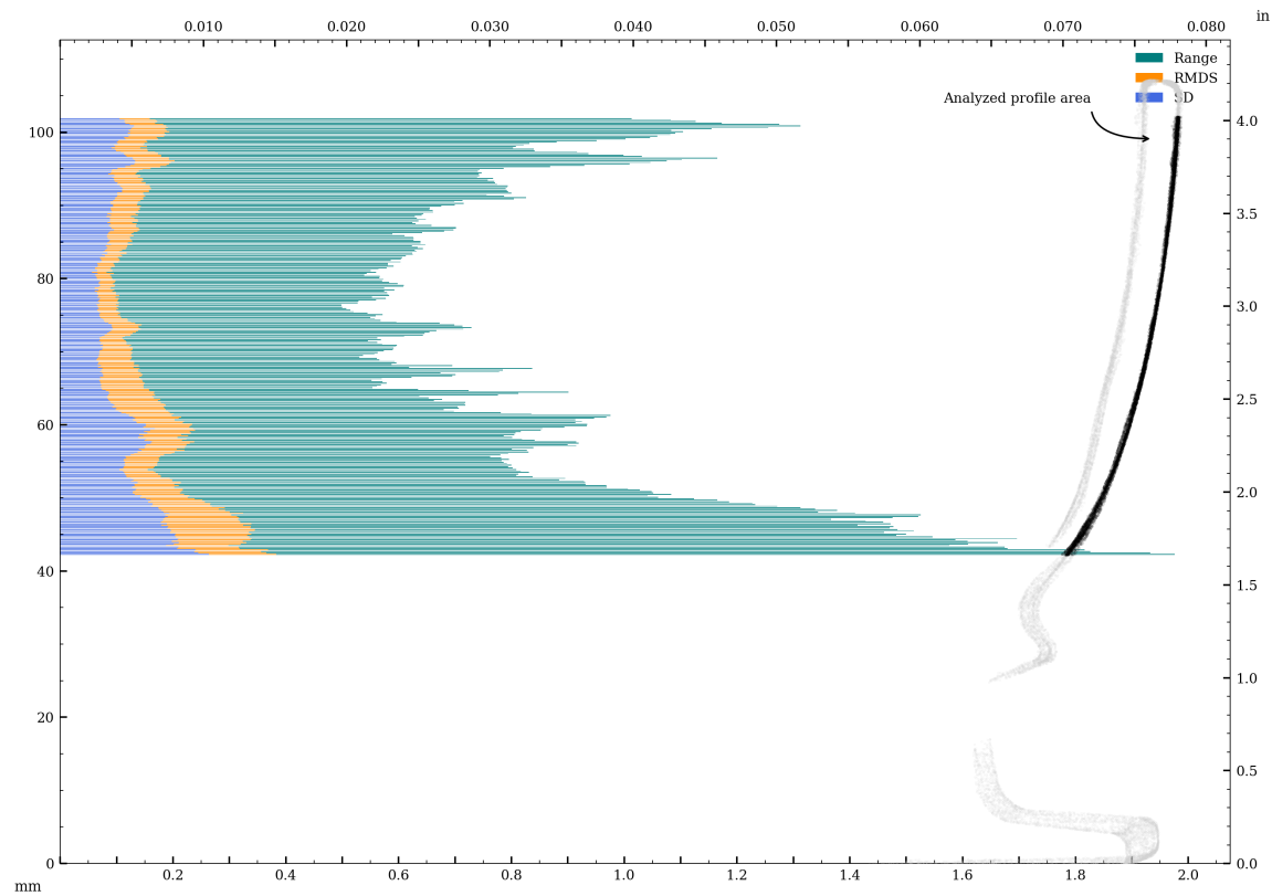
Figure 69: Circularity of exterior surface - in z-plane.
