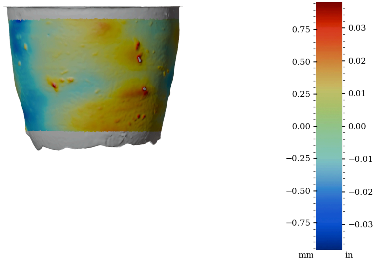
Figure 55: Surface variability heatmap of HV007, rotated 180°
