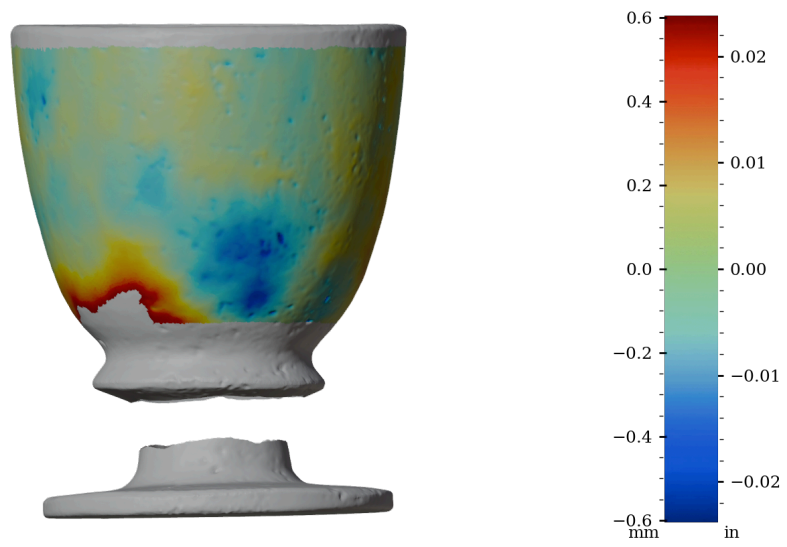
Figure 51: Surface variability heatmap of HV007, rotated 180°
