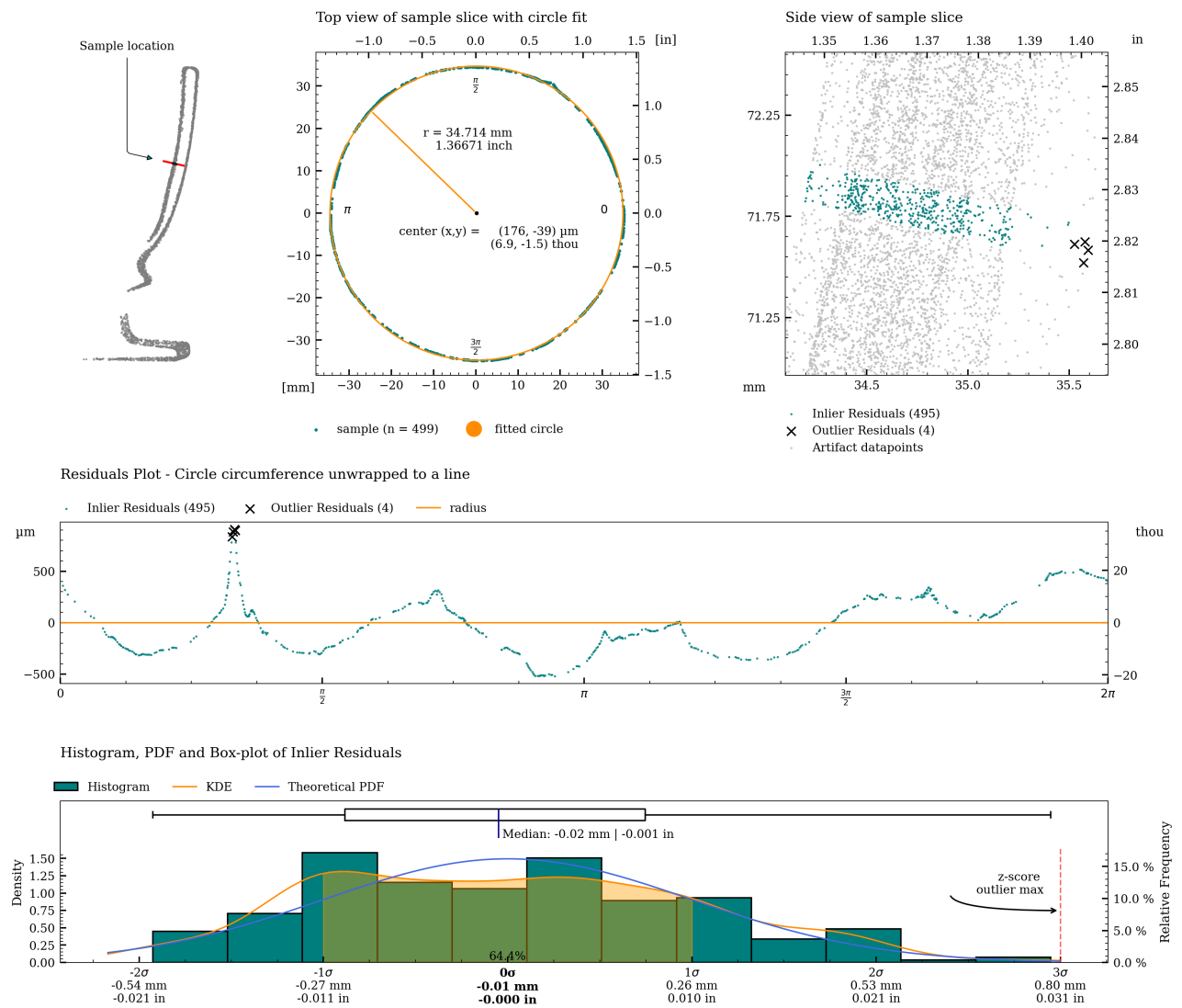
Figure 45: Detailed plot of concentricity measurement for c08_s.
