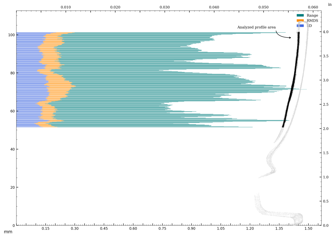
Figure 77: Circularity of interior_separate surface - in z-plane.
