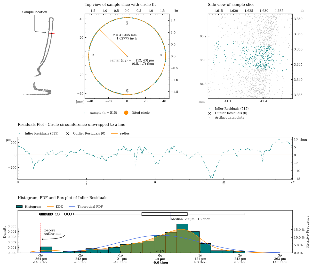
Figure 36: Detailed plot of concentricity measurement for c02.
