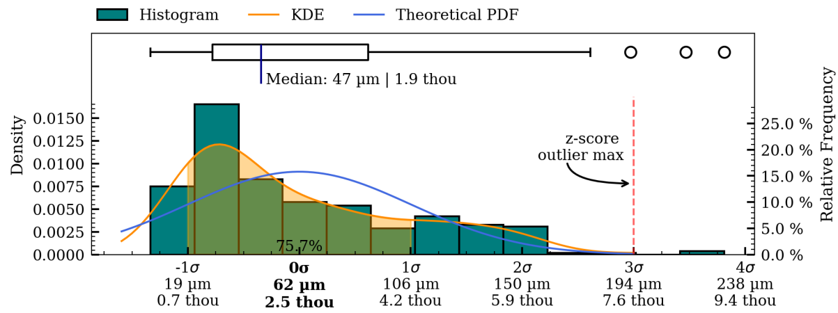
Figure 46: Coaxiality residual plots of exterior surface, HV007.
