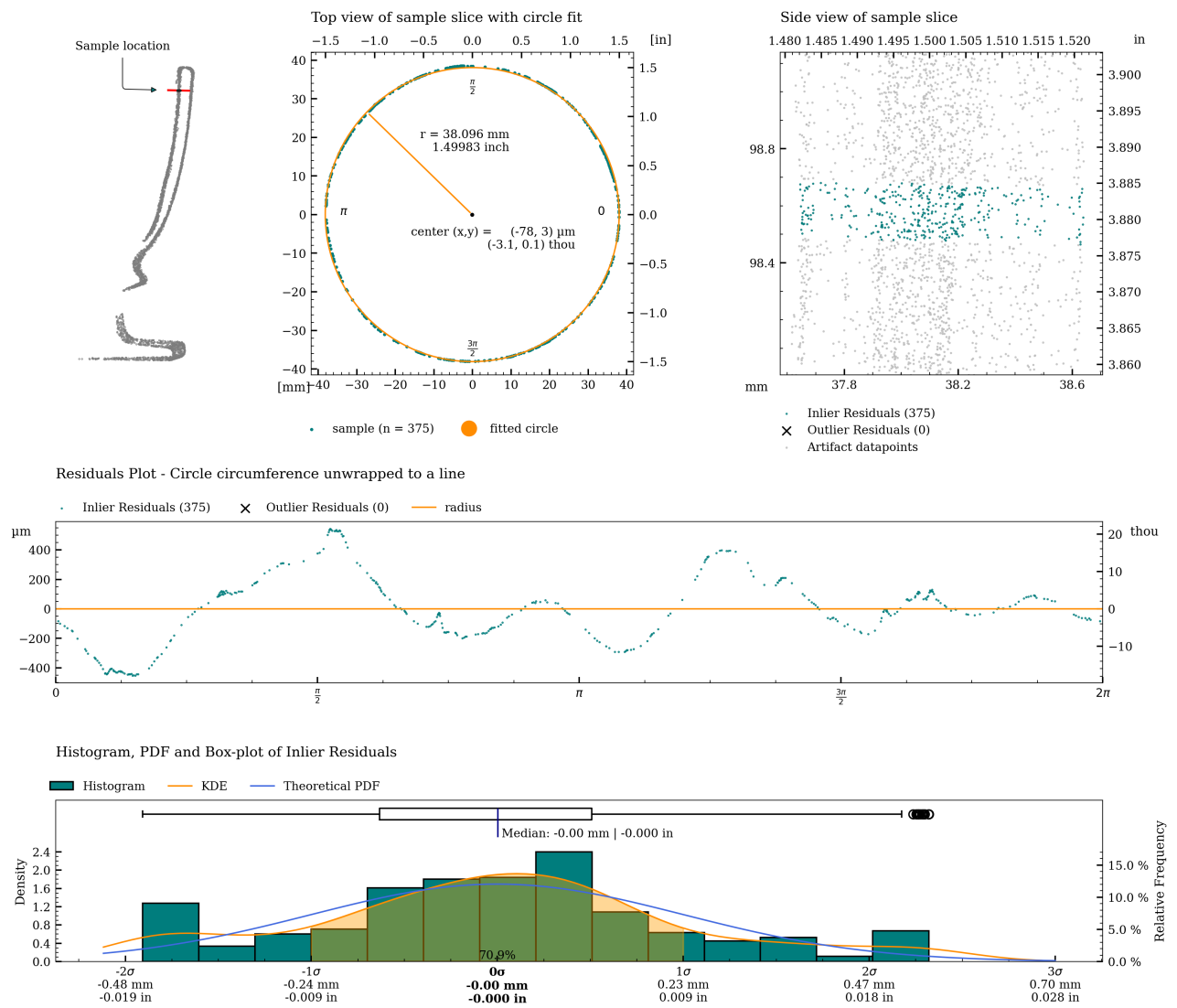
Figure 41: Detailed plot of concentricity measurement for c06_s.
