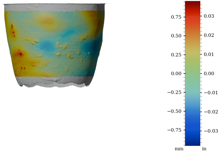
Figure 56: Surface variability heatmap of HV007, rotated 270°
