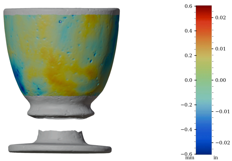
Figure 52: Surface variability heatmap of HV007, rotated 270°
