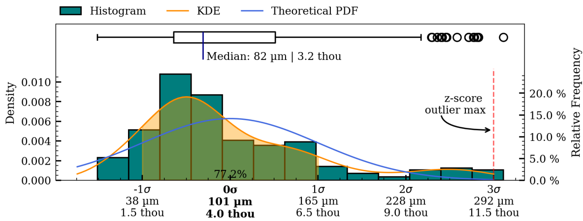
Figure 47: Coaxiality residual plots of interior surface, HV007.
