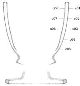
Figure 80: Circularity measurement sample locations, full mesh aligned to exterior surface
