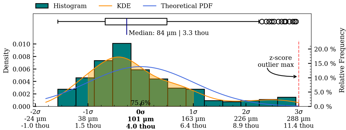
Figure 48: Coaxiality residual plots of interior_separate surface, HV007.
