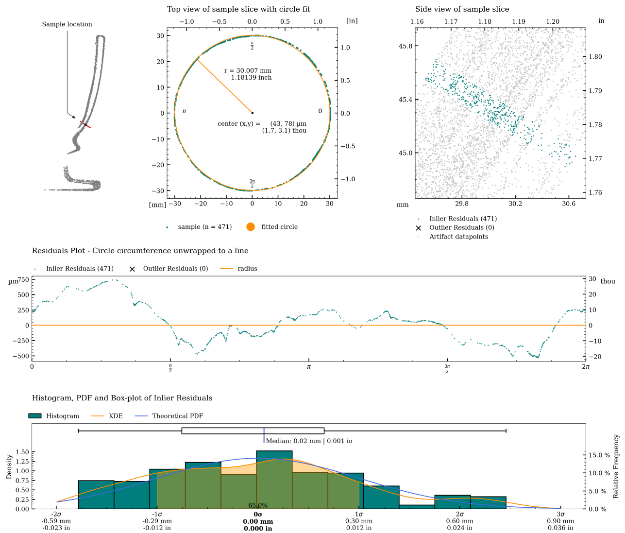
Figure 39: Detailed plot of concentricity measurement for c05.
