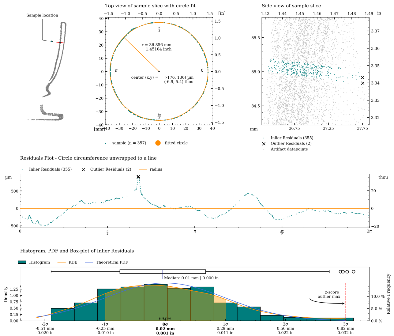
Figure 42: Detailed plot of concentricity measurement for c07.
