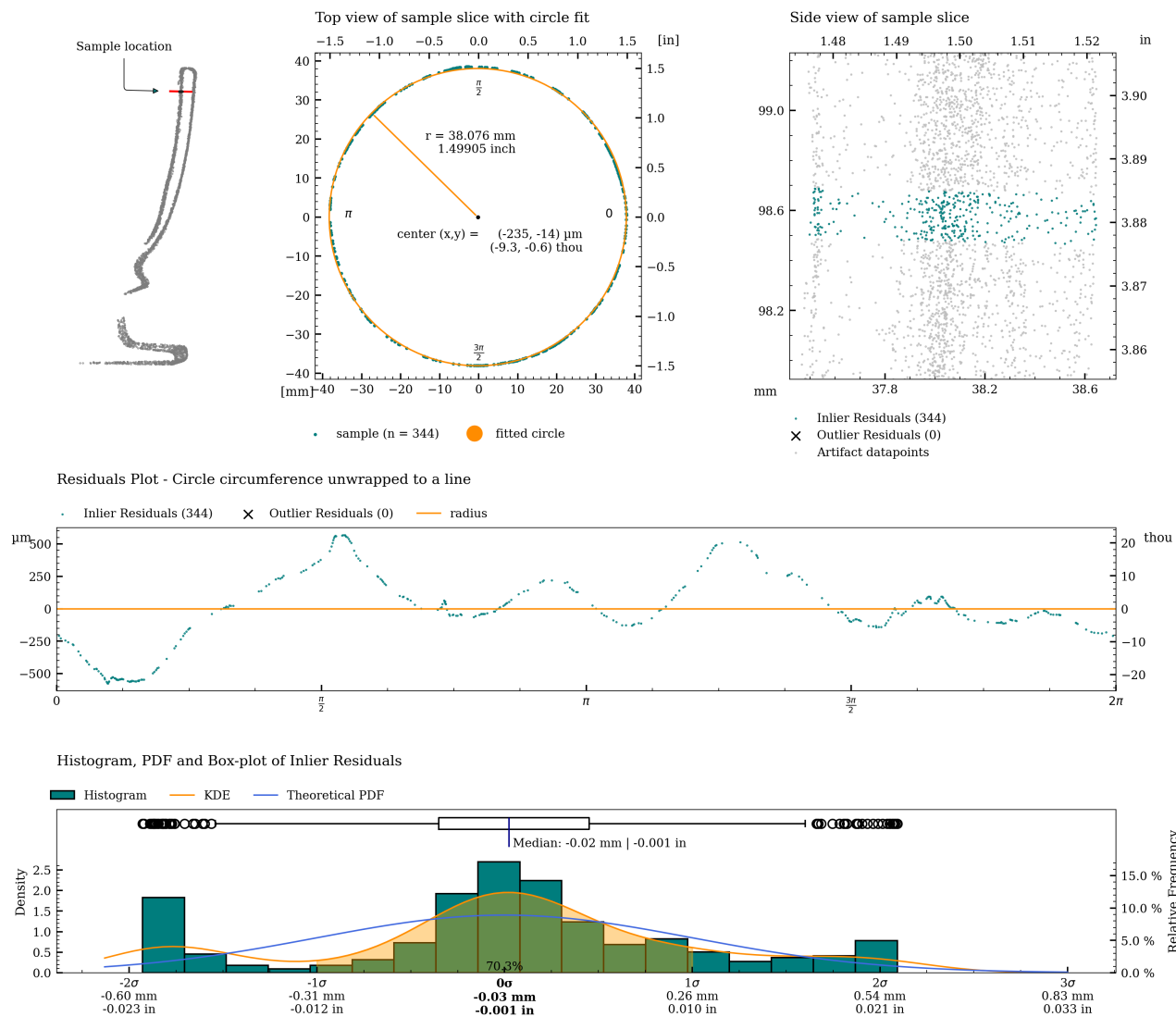
Figure 40: Detailed plot of concentricity measurement for c06.
