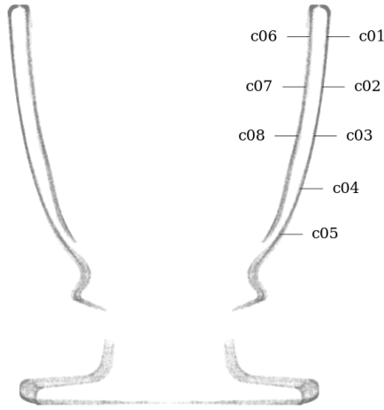
Figure 64: Circularity measurement sample locations, full mesh aligned to exterior surface
