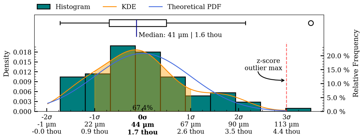
Figure 39: Coaxiality residual plots of interior surface, HV006.
