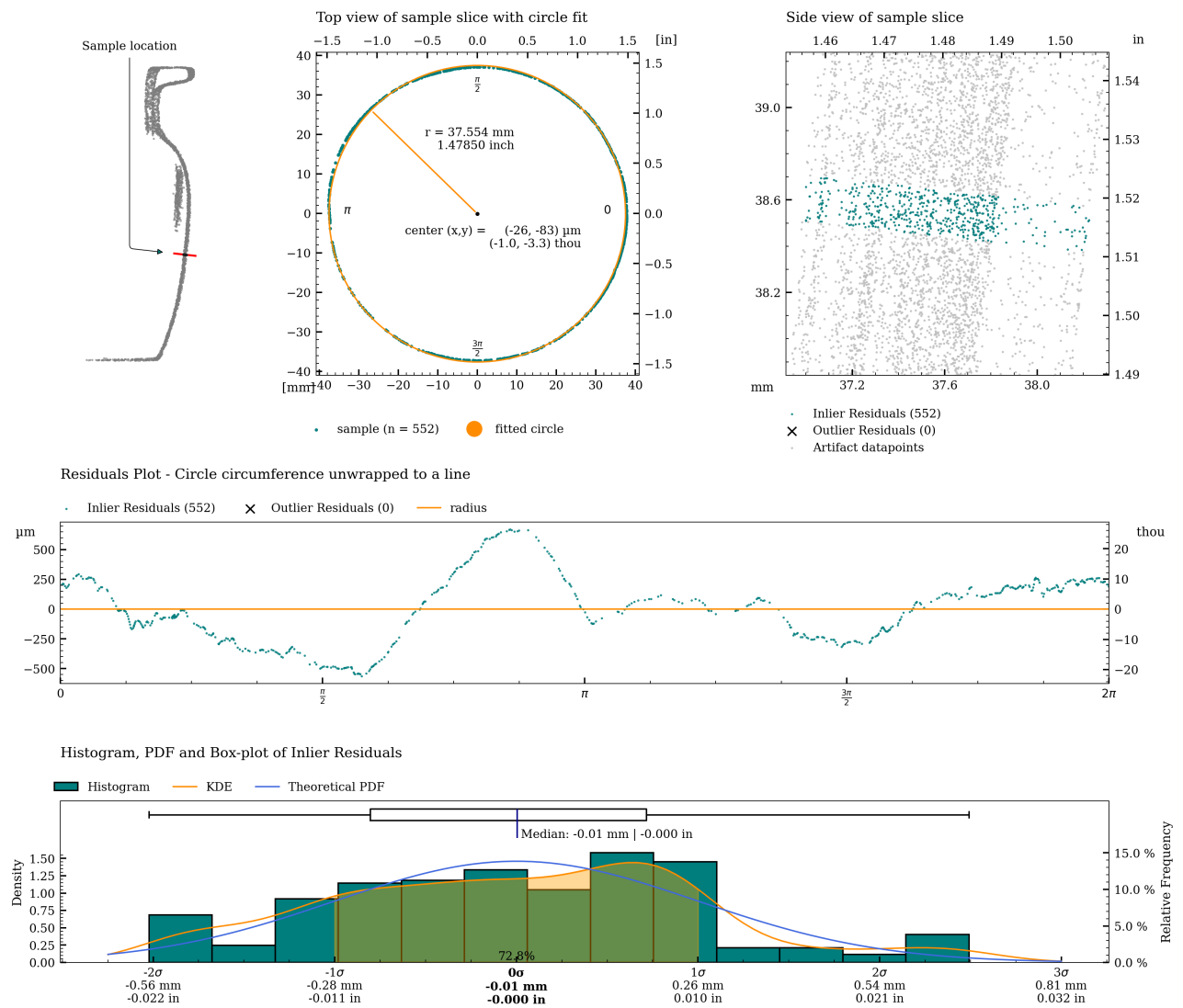
Figure 34: Detailed plot of concentricity measurement for c04.
