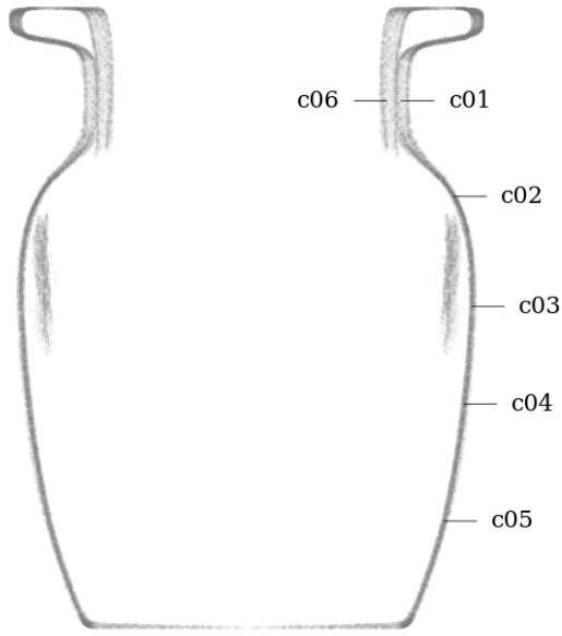
Figure 58: Circularity measurement sample locations, full mesh aligned to exterior surface
