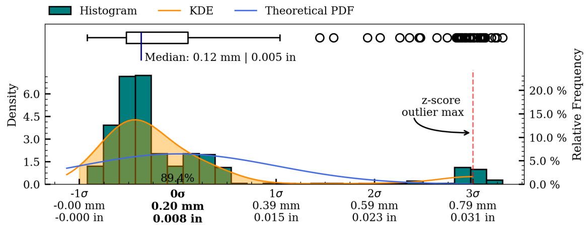
Figure 38: Coaxiality residual plots of exterior surface, HV006.
