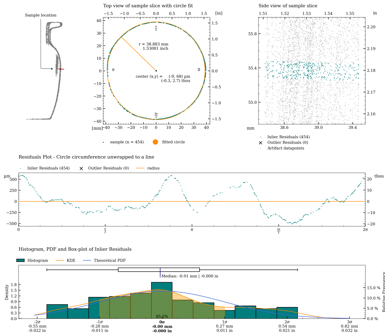
Figure 33: Detailed plot of concentricity measurement for c03.
