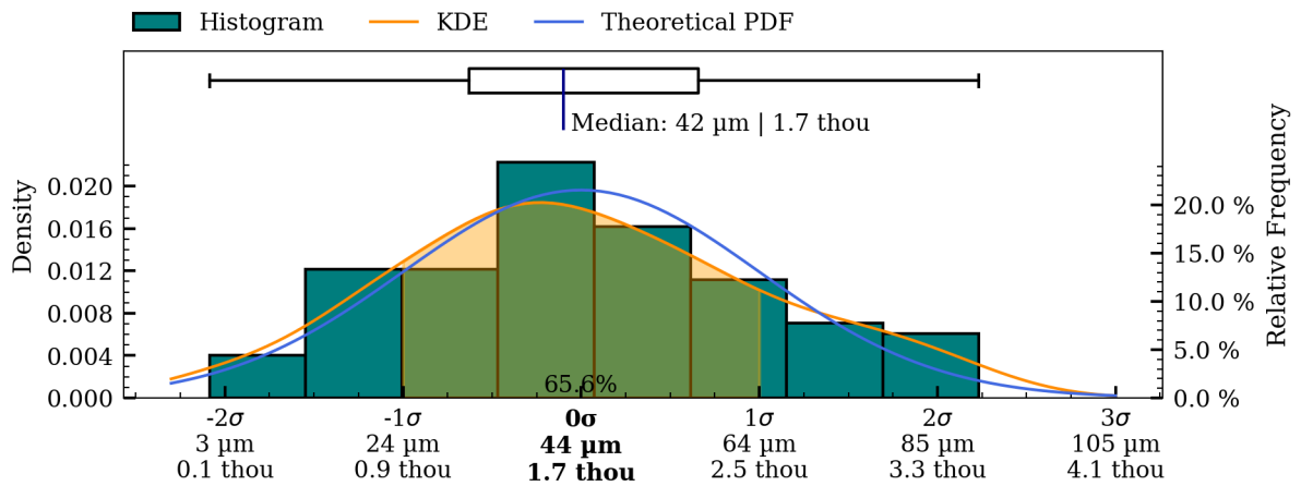
Figure 40: Coaxiality residual plots of interior_separate surface, HV006.
