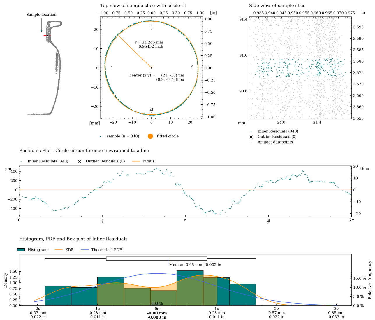
Figure 37: Detailed plot of concentricity measurement for c06_s.
