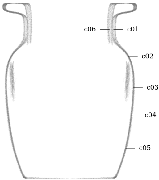
Figure 29: Circularity measurement sample locations, full mesh aligned to exterior surface
