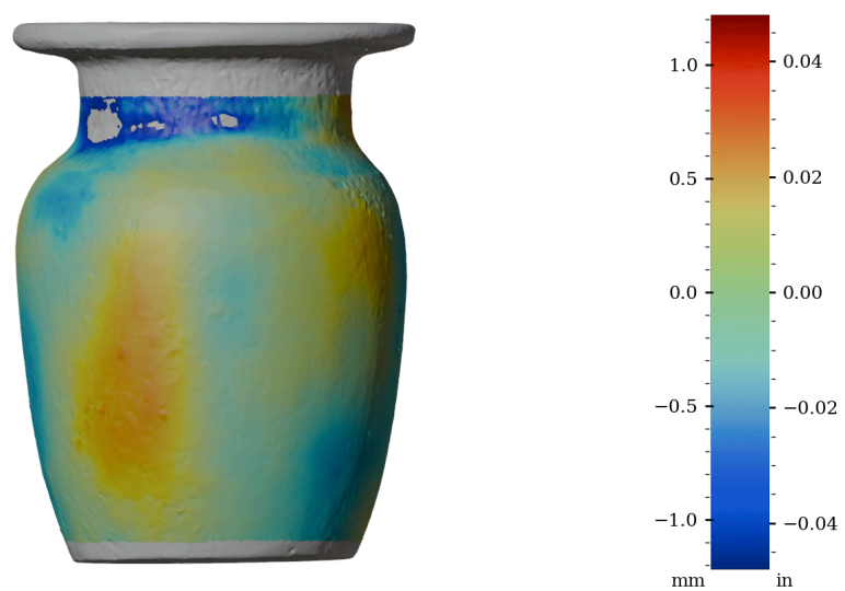
Figure 44: Surface variability heatmap of HV006, rotated 270°
