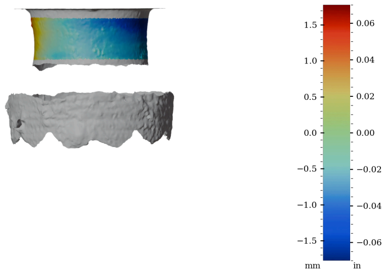
Figure 47: Surface variability heatmap of HV006, rotated 180°
