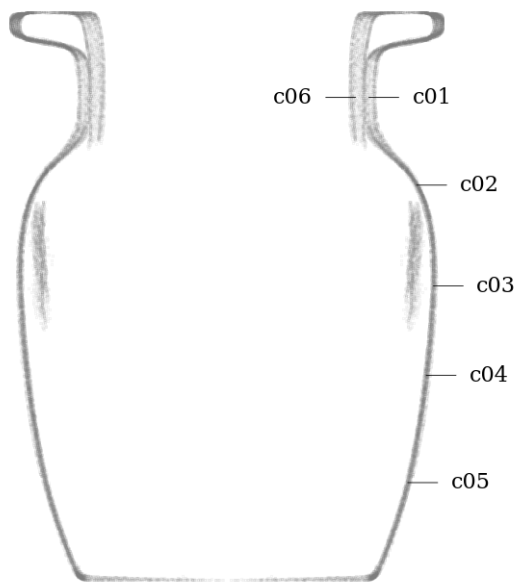
Figure 74: Circularity measurement sample locations, full mesh aligned to exterior surface
