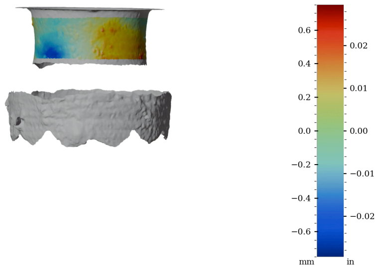
Figure 51: Surface variability heatmap of HV006, rotated 180°
