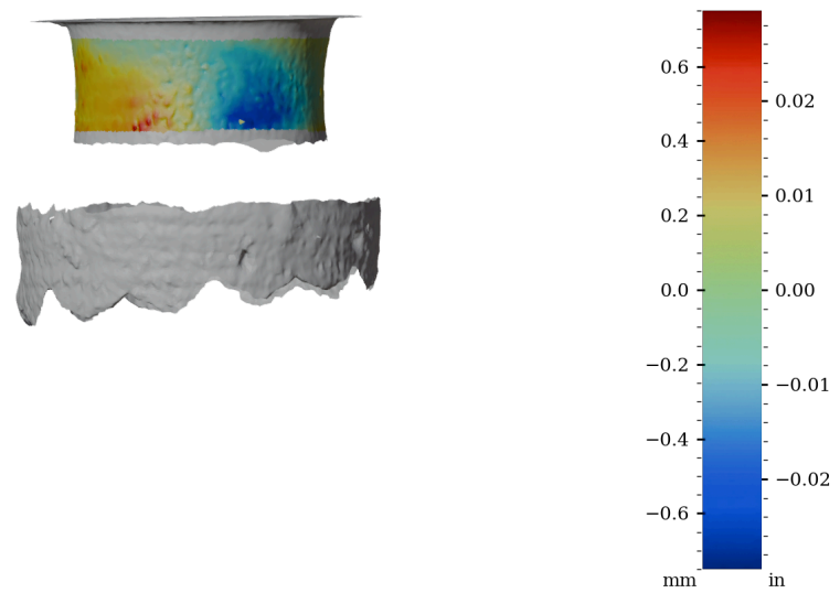
Figure 52: Surface variability heatmap of HV006, rotated 270°
