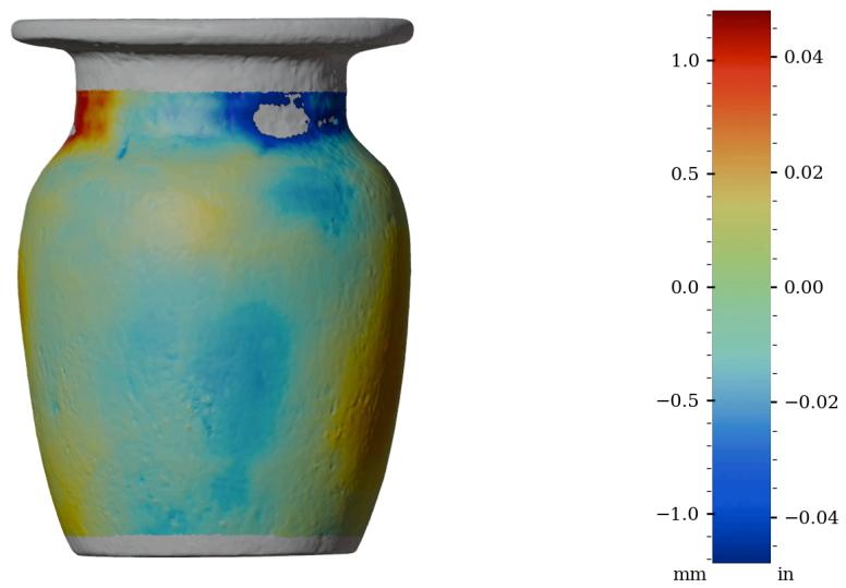
Figure 43: Surface variability heatmap of HV006, rotated 180°
