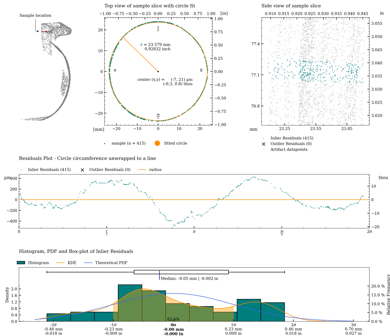
Figure 39: Detailed plot of concentricity measurement for c06_s.
