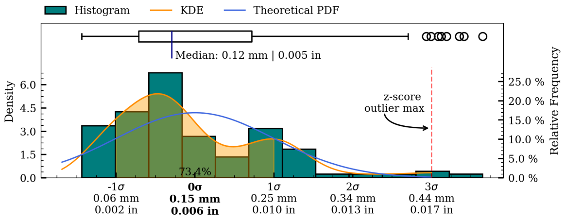
Figure 42: Coaxiality residual plots of exterior surface, HV003.
