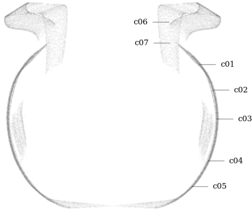
Figure 31: Circularity measurement sample locations, full mesh aligned to exterior surface
