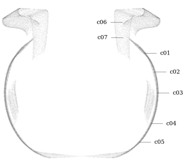
Figure 62: Circularity measurement sample locations, full mesh aligned to exterior surface
