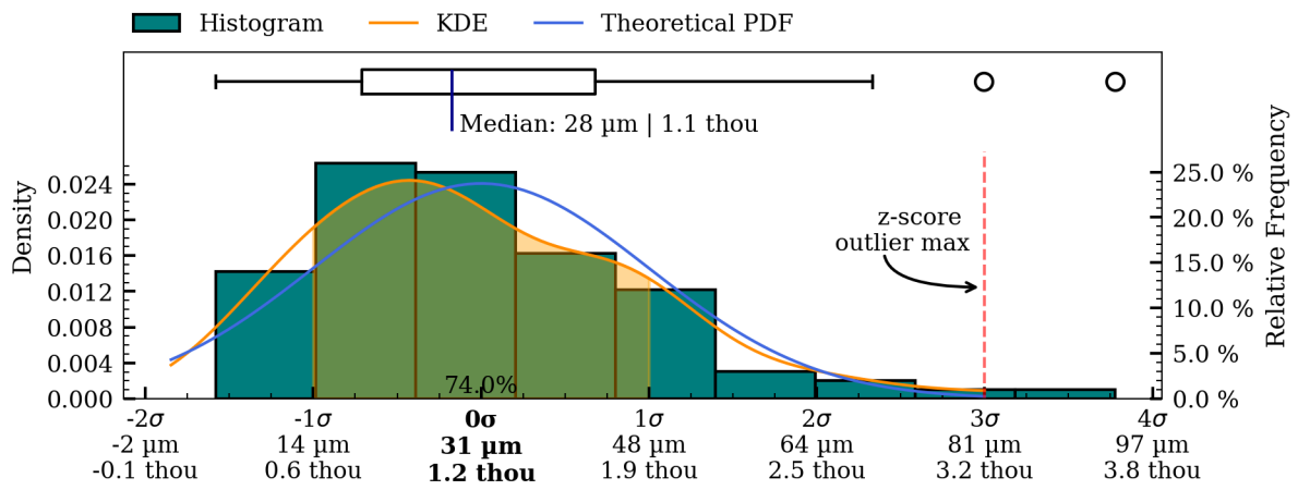
Figure 44: Coaxiality residual plots of interior_separate surface, HV003.
