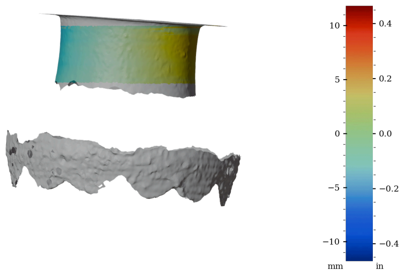
Figure 52: Surface variability heatmap of HV003, rotated 270°
