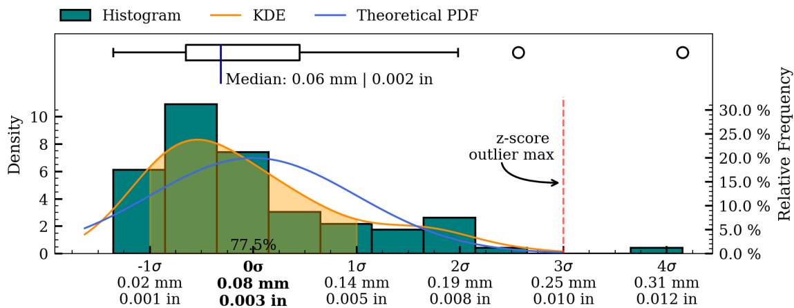
Figure 43: Coaxiality residual plots of interior surface, HV003.
