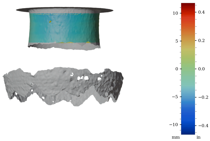
Figure 51: Surface variability heatmap of HV003, rotated 180°
