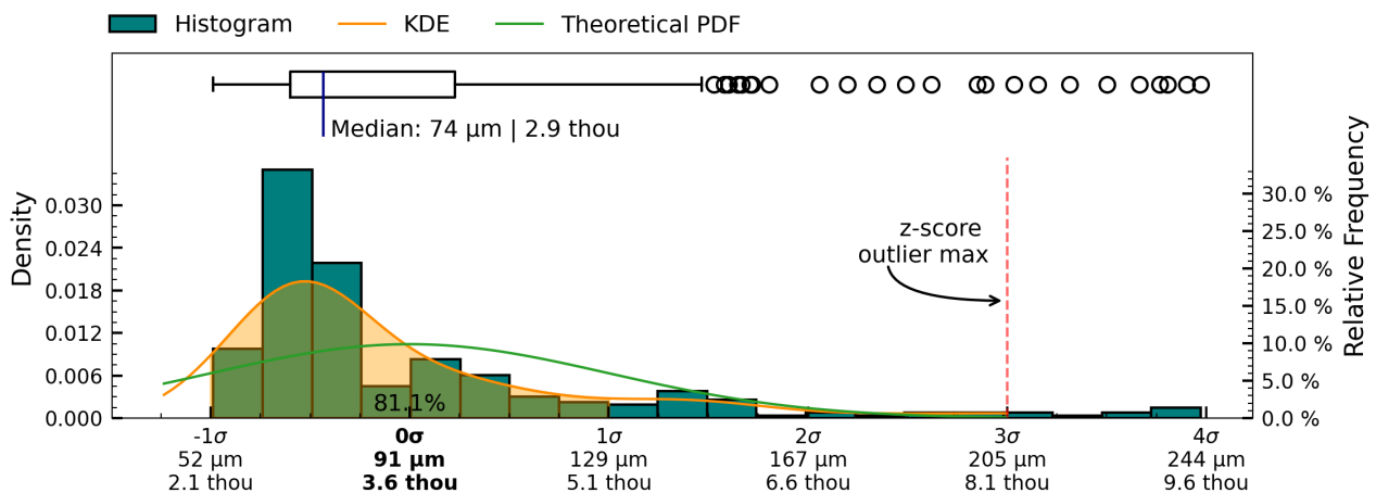
Figure 17: Root Mean Squared Deviation measurement distribution across measured slices of exterior surface
