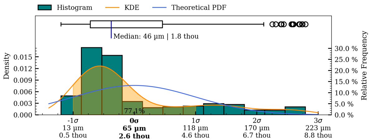
Figure 38: Coaxiality residual plots of exterior surface, HV002.
