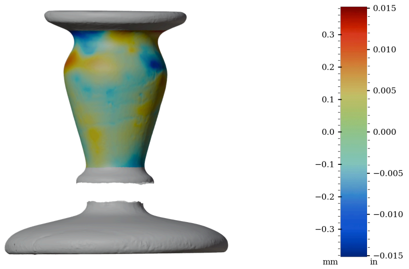
Figure 43: Surface variability heatmap of HV002, rotated 180°
