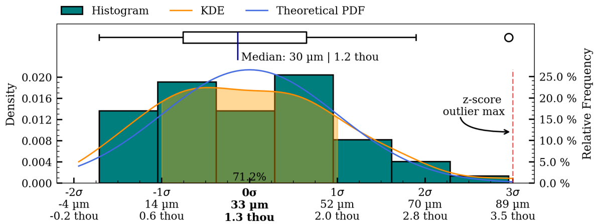
Figure 39: Coaxiality residual plots of interior surface, HV002.
