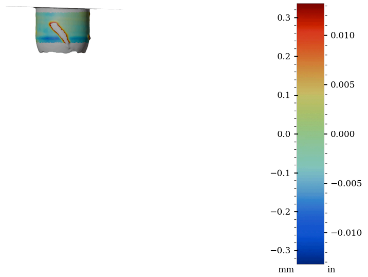
Figure 51: Surface variability heatmap of HV002, rotated 180°
