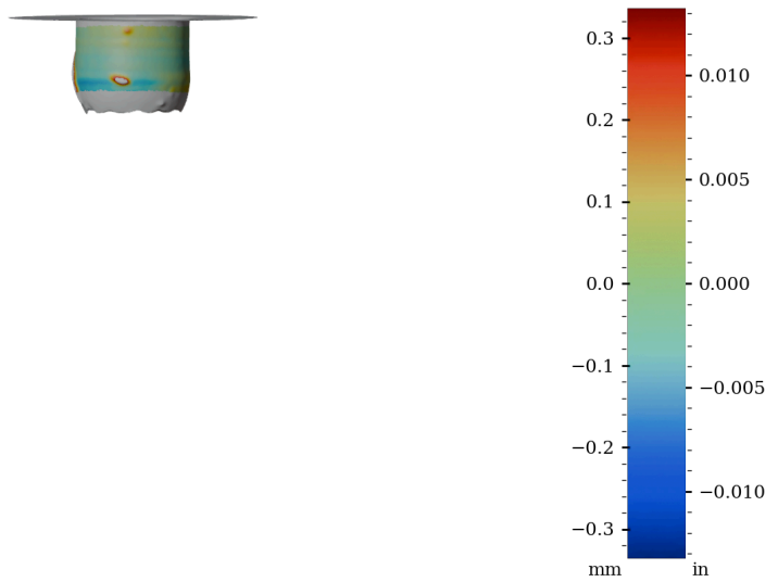
Figure 52: Surface variability heatmap of HV002, rotated 270°
