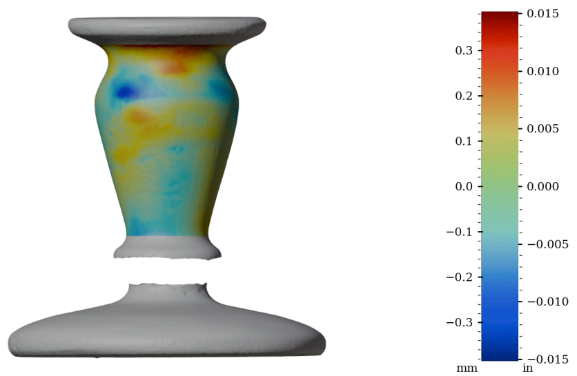
Figure 44: Surface variability heatmap of HV002, rotated 270°
