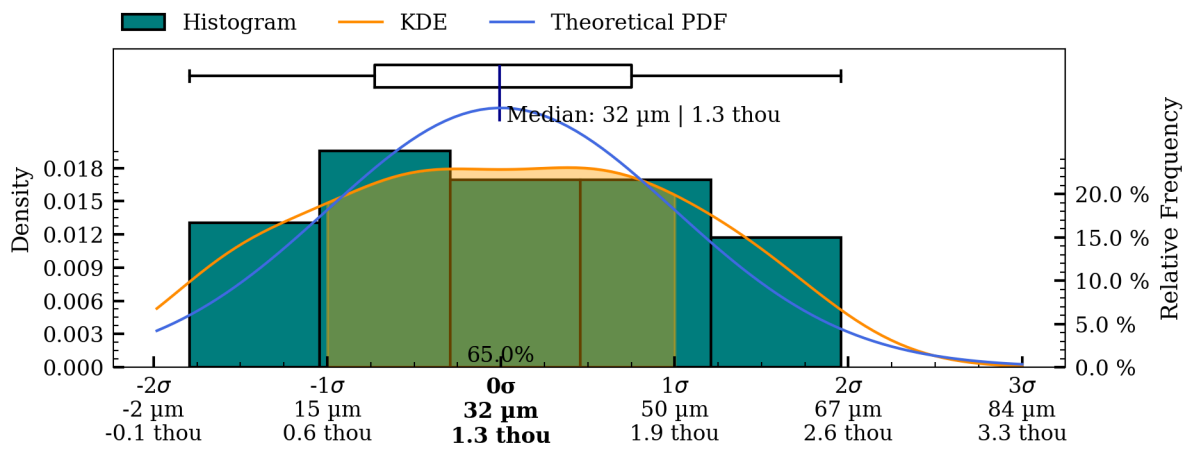
Figure 40: Coaxiality residual plots of interior_separate surface, HV002.
