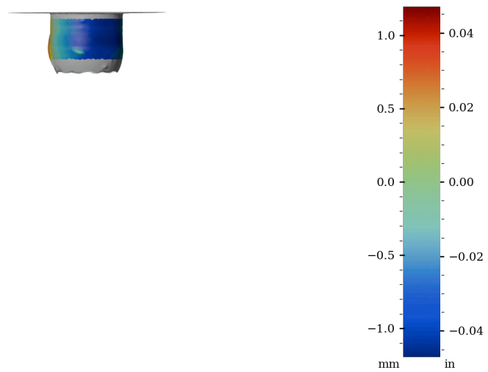
Figure 48: Surface variability heatmap of HV002, rotated 270°
