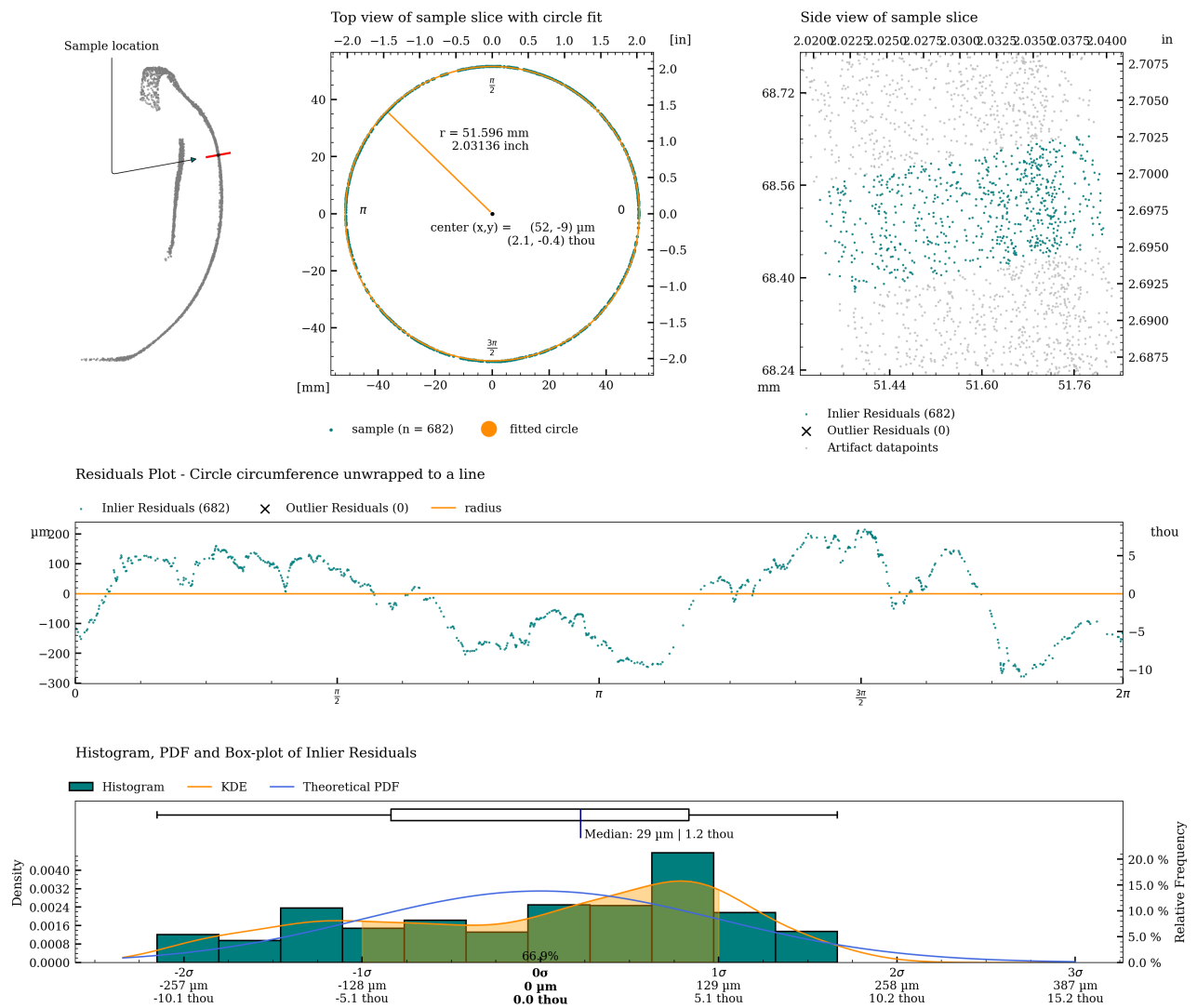
Figure 34: Detailed plot of concentricity measurement for c02.
