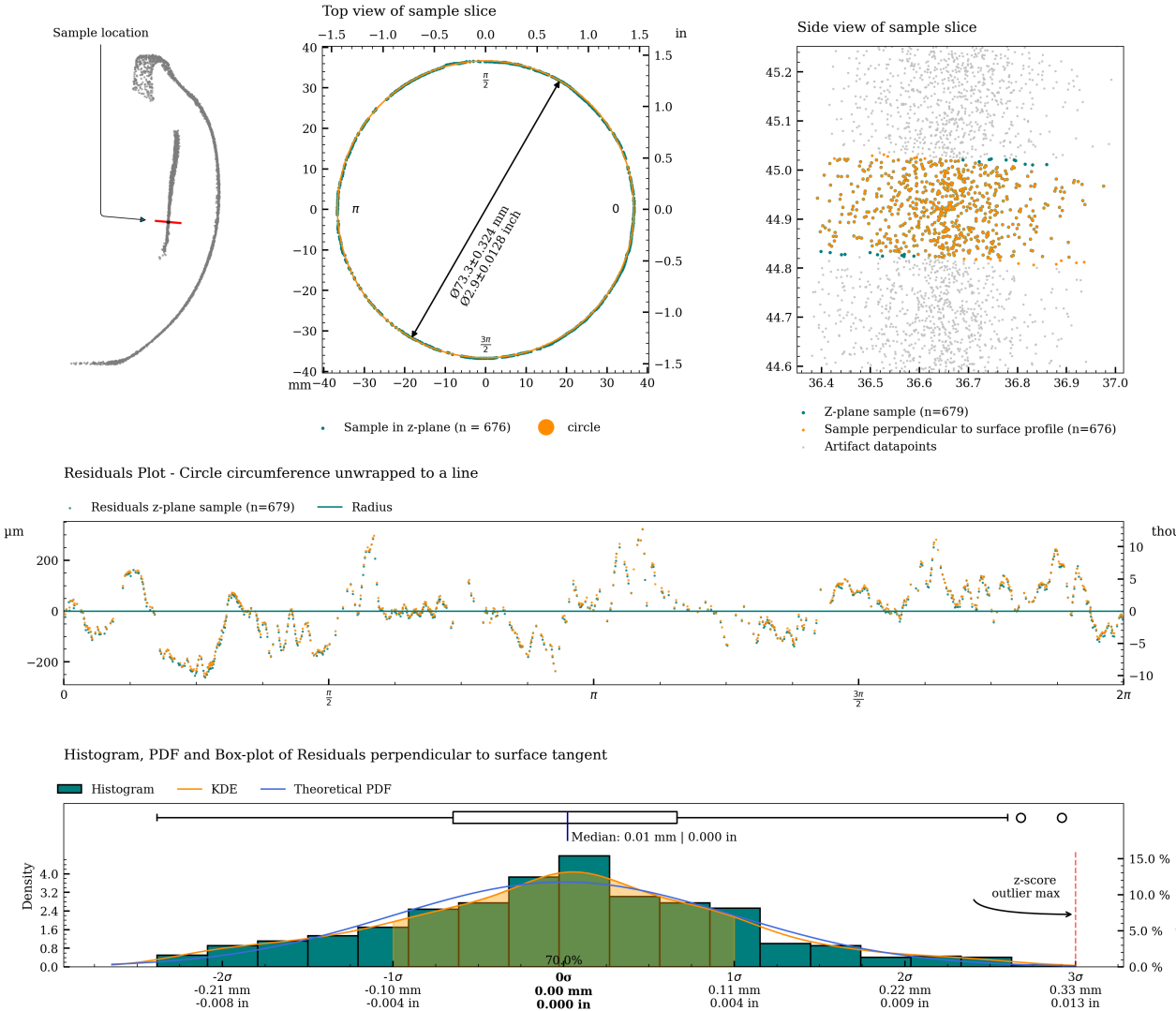
Figure 14: Charts with statistics for the measurement of c08_s
