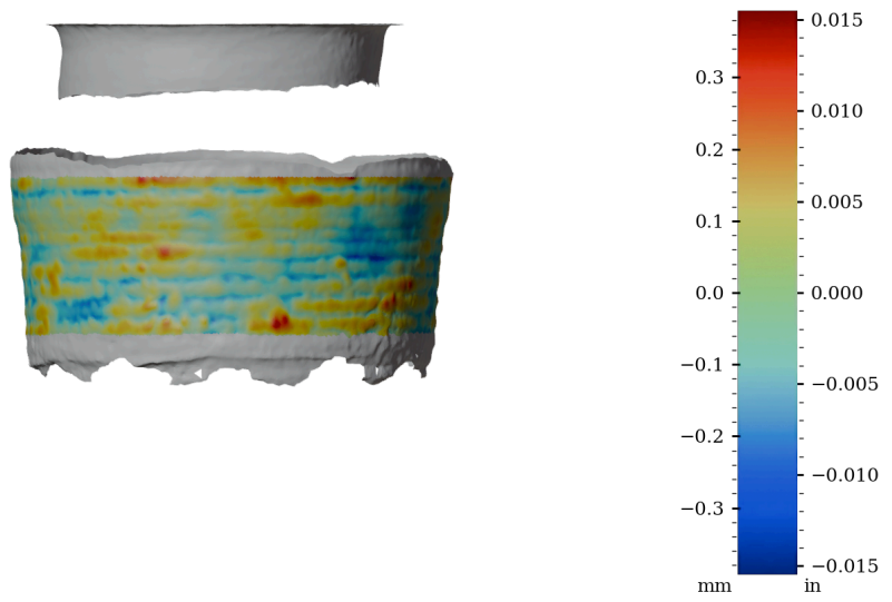
Figure 55: Surface variability heatmap of HV001, rotated 180°
