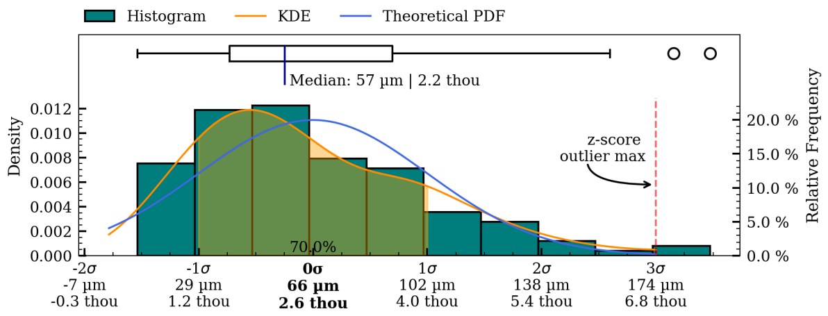
Figure 43: Coaxiality residual plots of interior surface, HV001.
