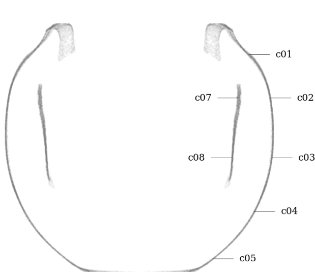
Figure 78: Circularity measurement sample locations, full mesh aligned to exterior surface
