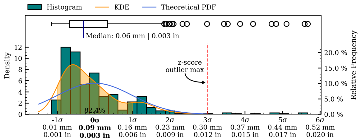
Figure 42: Coaxiality residual plots of exterior surface, HV001.
