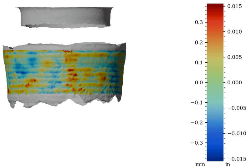
Figure 56: Surface variability heatmap of HV001, rotated 270°
