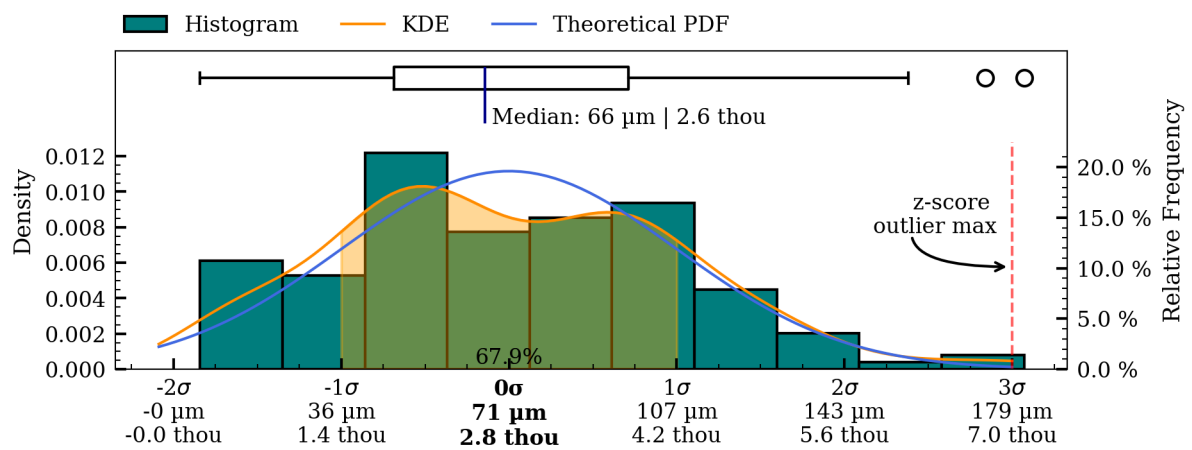
Figure 44: Coaxiality residual plots of interior_separate surface, HV001.
