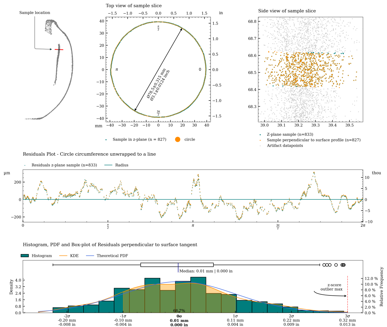
Figure 12: Charts with statistics for the measurement of c07_s.
