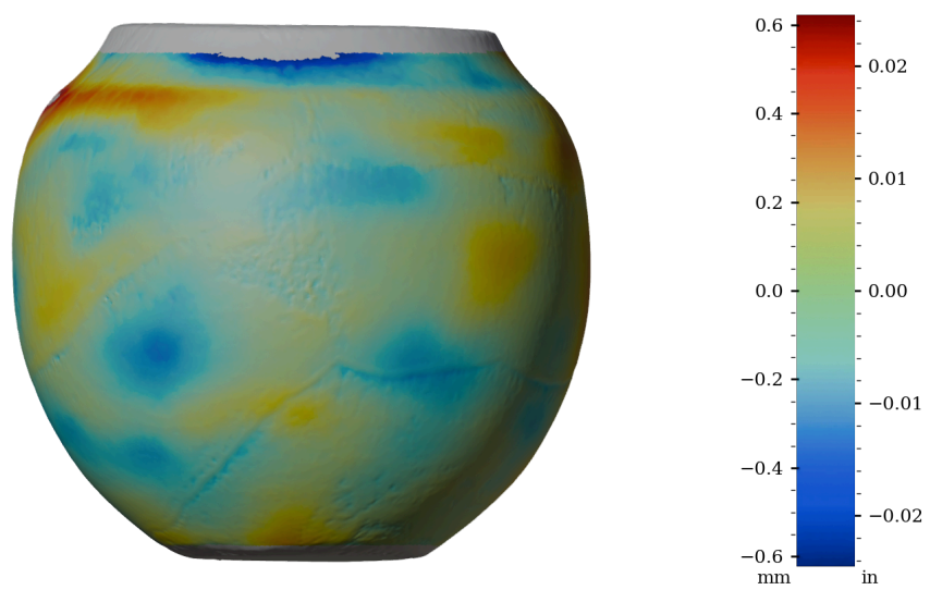
Figure 48: Surface variability heatmap of HV001, rotated 270°
