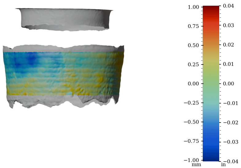
Figure 52: Surface variability heatmap of HV001, rotated 270°
