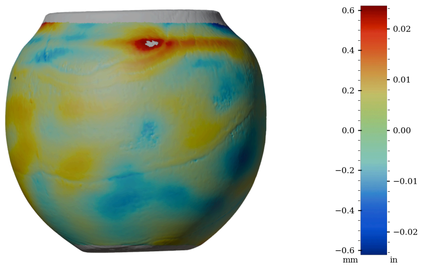
Figure 47: Surface variability heatmap of HV001, rotated 180°
