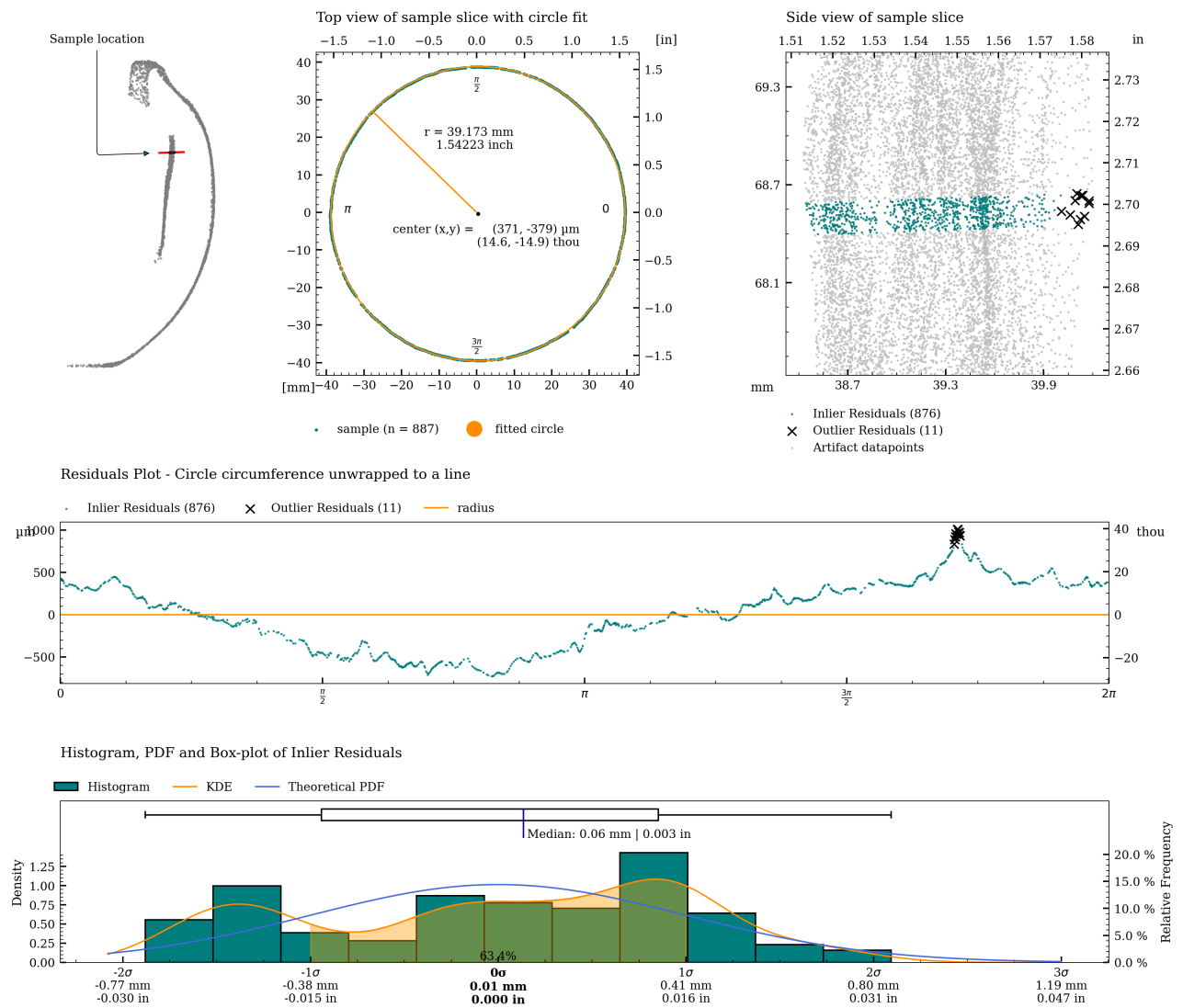
Figure 38: Detailed plot of concentricity measurement for c07.
