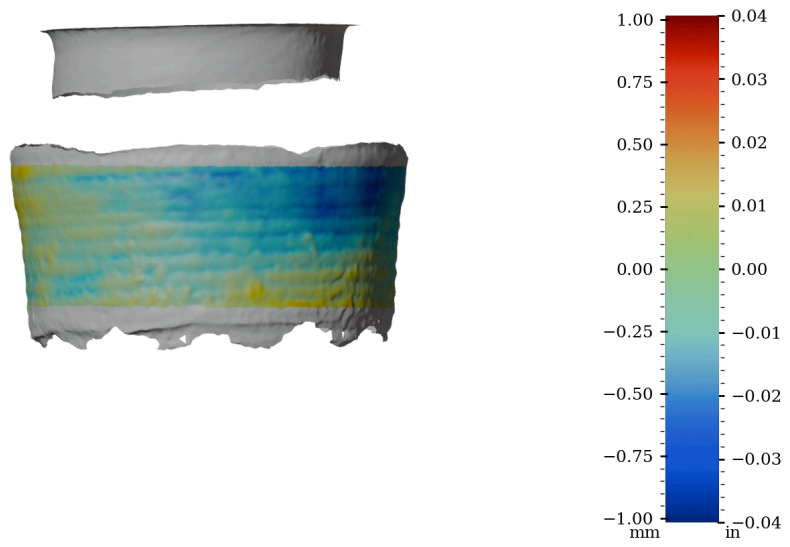
Figure 51: Surface variability heatmap of HV001, rotated 180°
