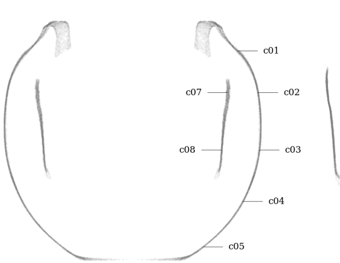
Figure 60: Circularity measurement sample locations, full mesh aligned to exterior surface
