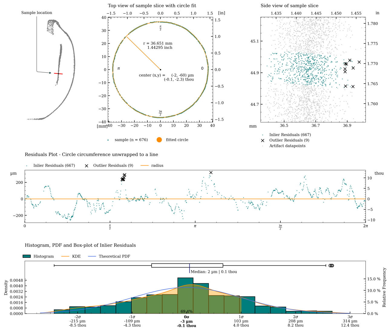
Figure 41: Detailed plot of concentricity measurement for c08_s.
