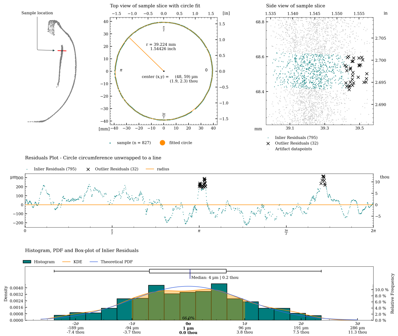
Figure 39: Detailed plot of concentricity measurement for c07_s.
