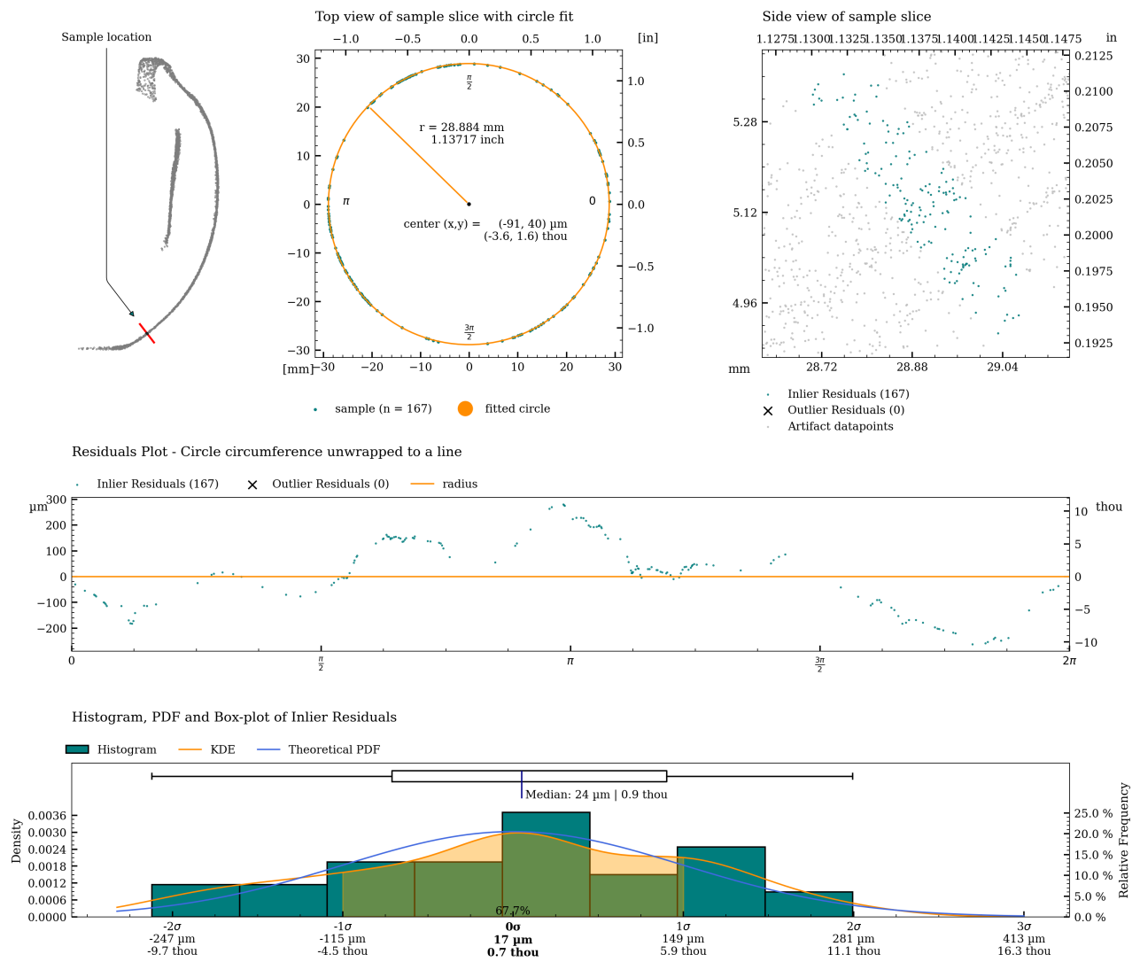
Figure 37: Detailed plot of concentricity measurement for c05.
