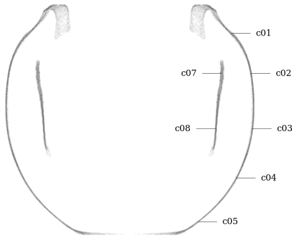
Figure 76: Circularity measurement sample locations, full mesh aligned to exterior surface
